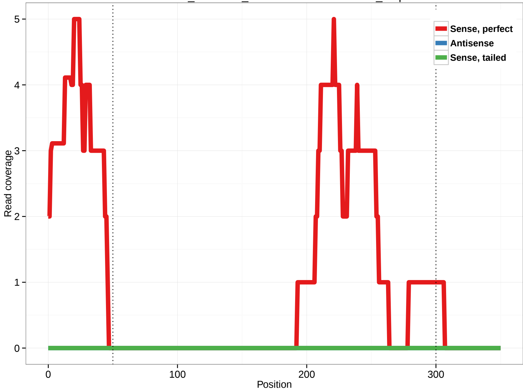
ornAna1_ensGene_ENSOANT00000006636_2.5p
