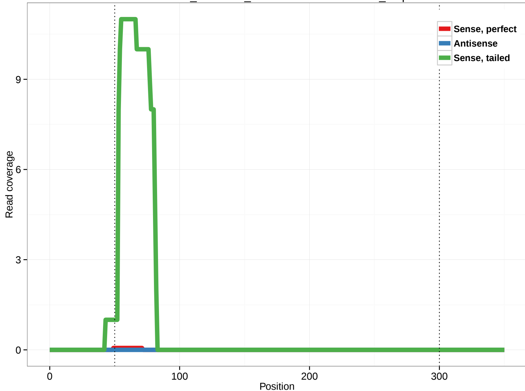
ornAna1_ensGene_ENSOANT00000006591_8.3p
