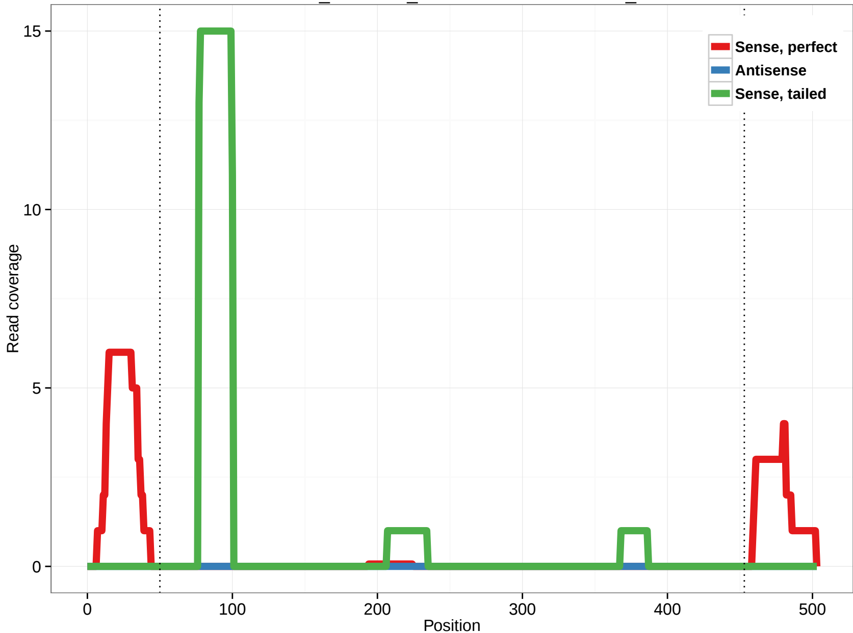
ornAna1_ensGene_ENSOANT00000006583_11
