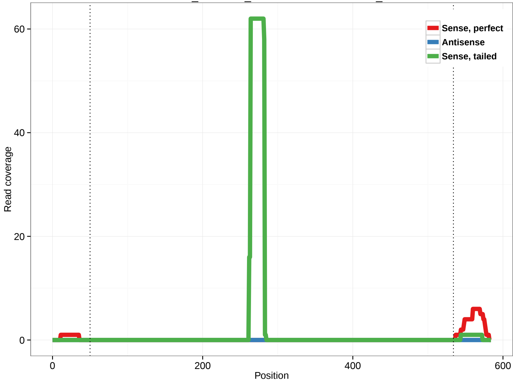
ornAna1_ensGene_ENSOANT00000006535_11
