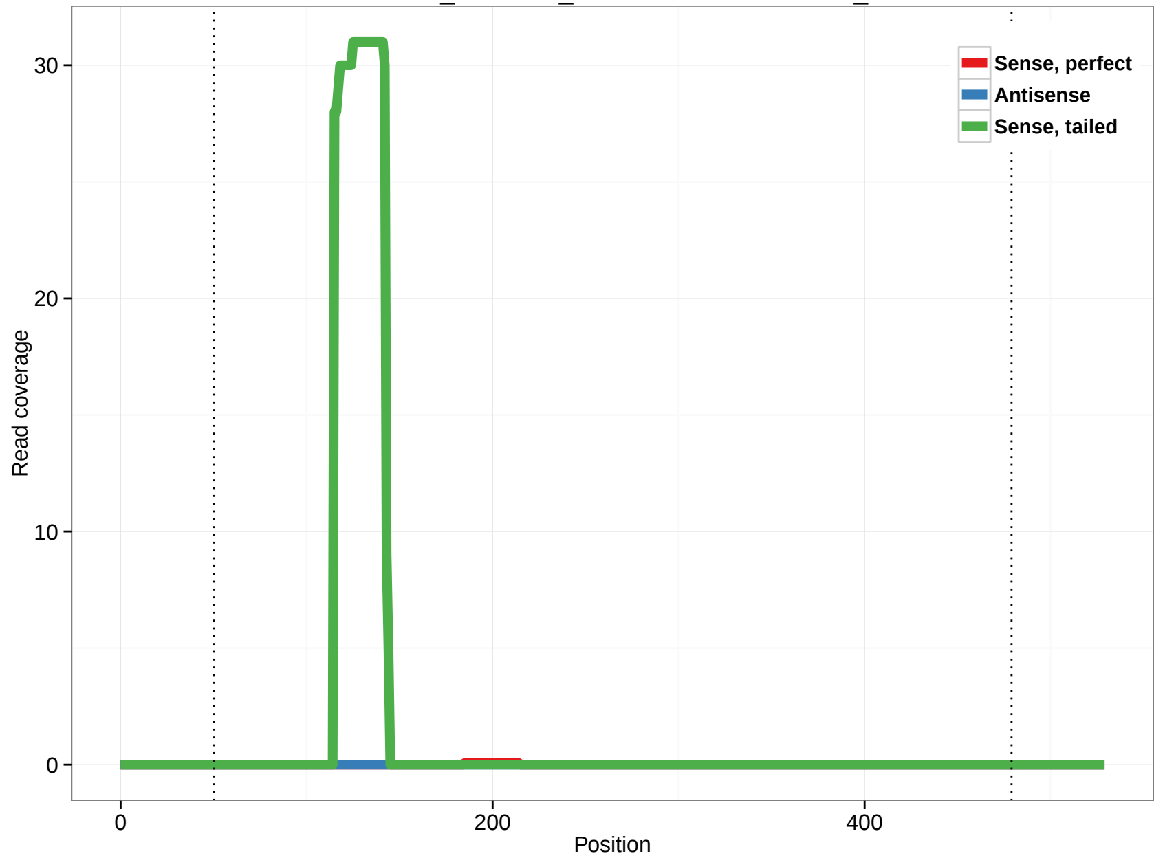
ornAna1_ensGene_ENSOANT00000006476_1
