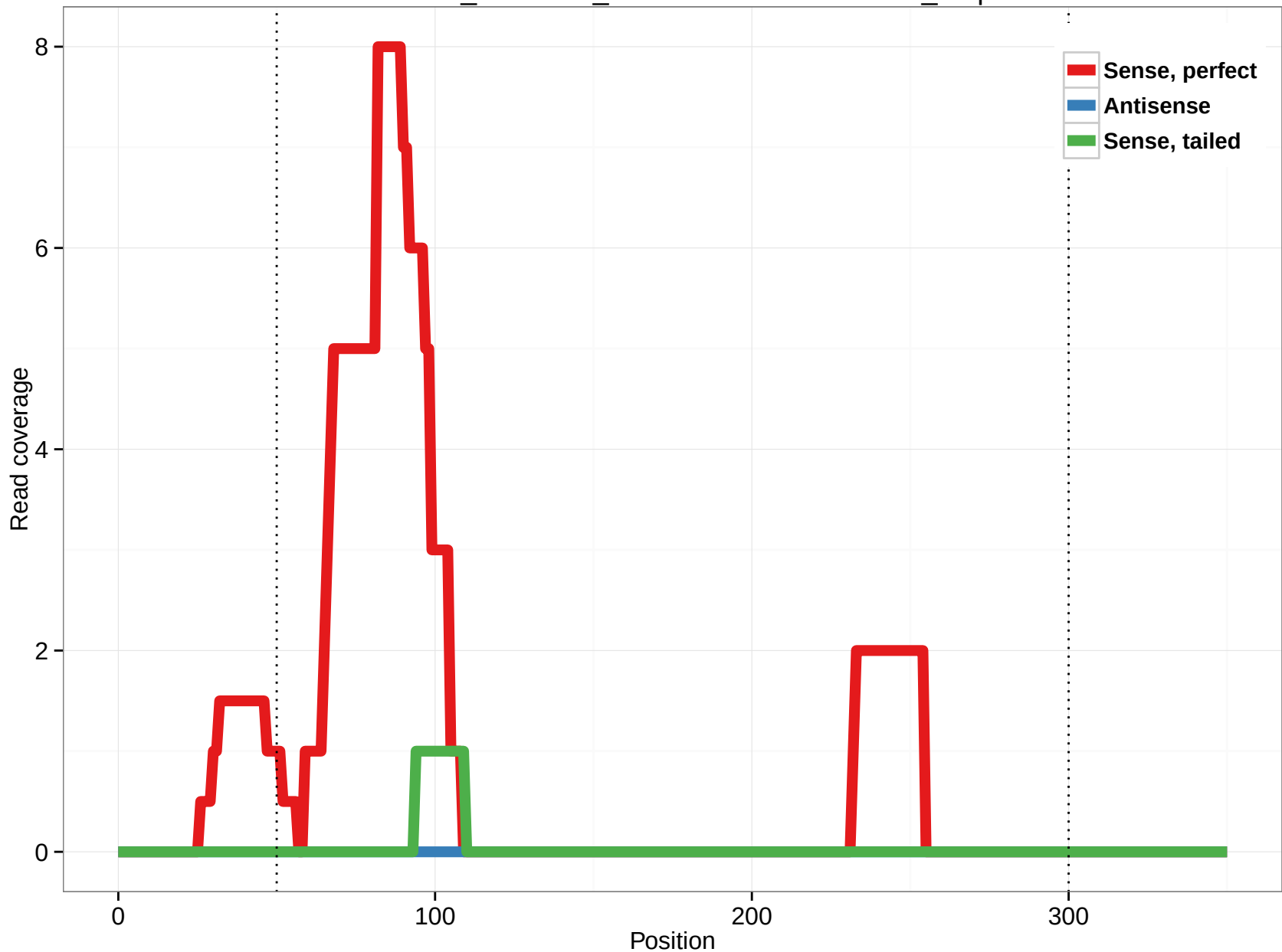
ornAna1_ensGene ENSOANT00000006469 5.3p
