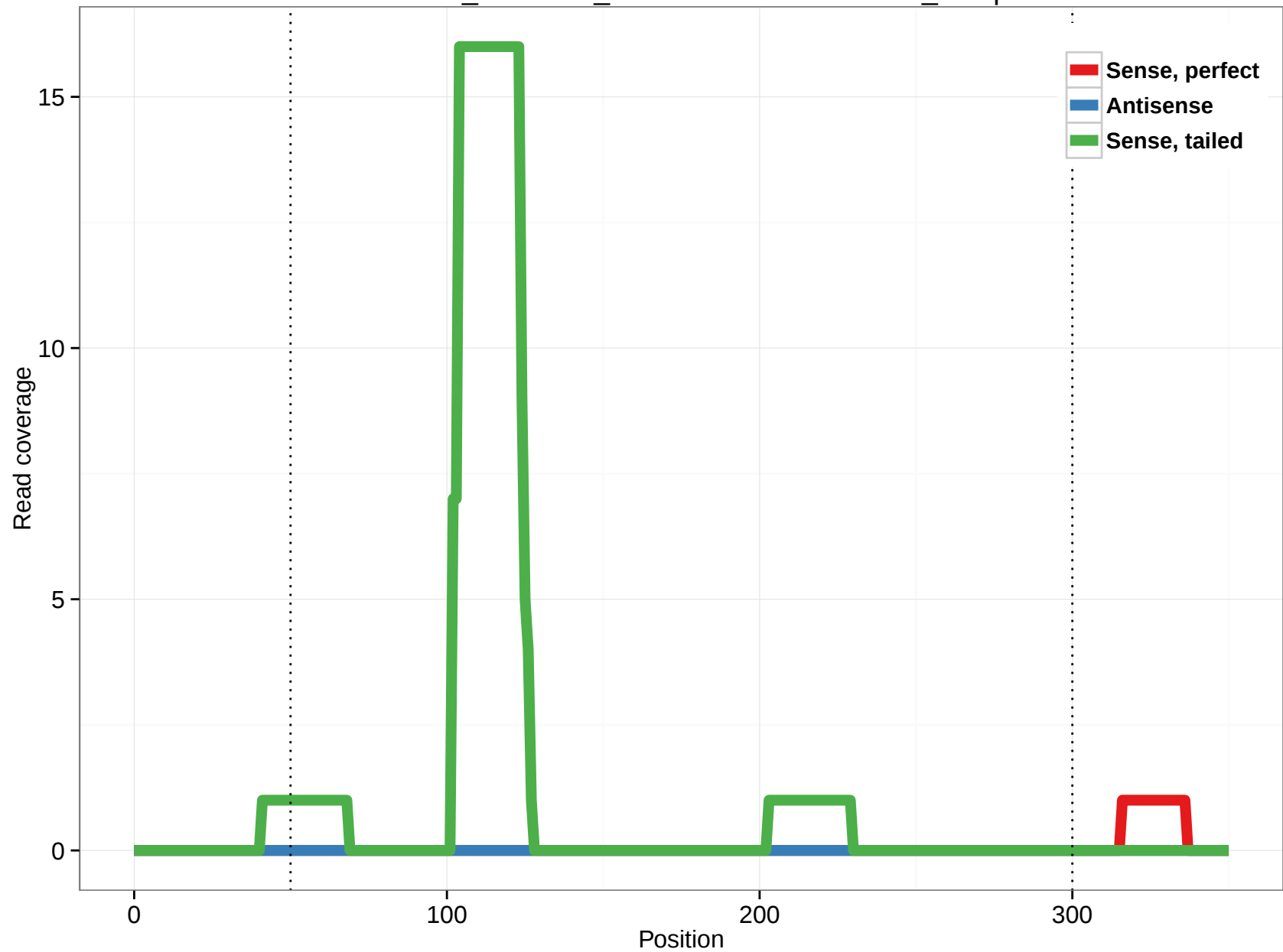
ornAna1_ensGene_ENSOANT00000006401_11.3p
