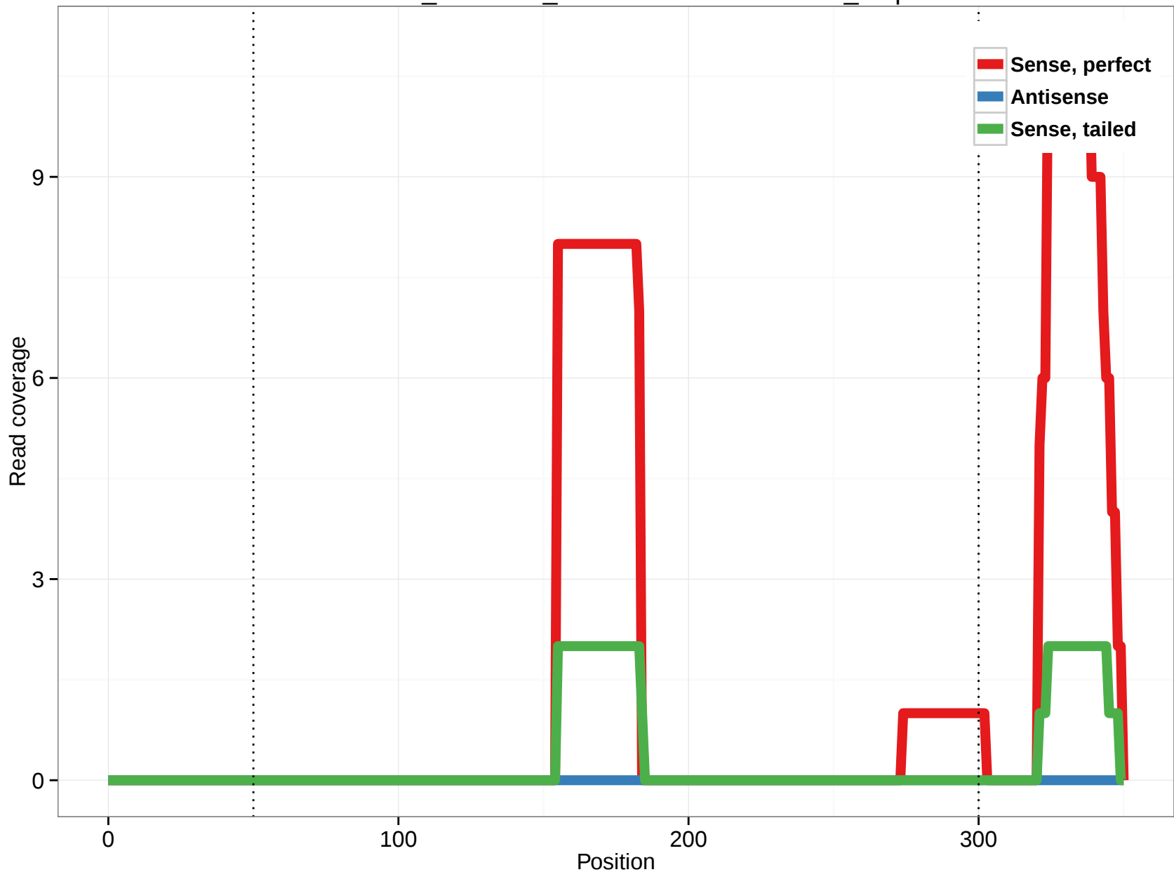
ornAna1_ensGene_ENSOANT00000006399_5.3p
