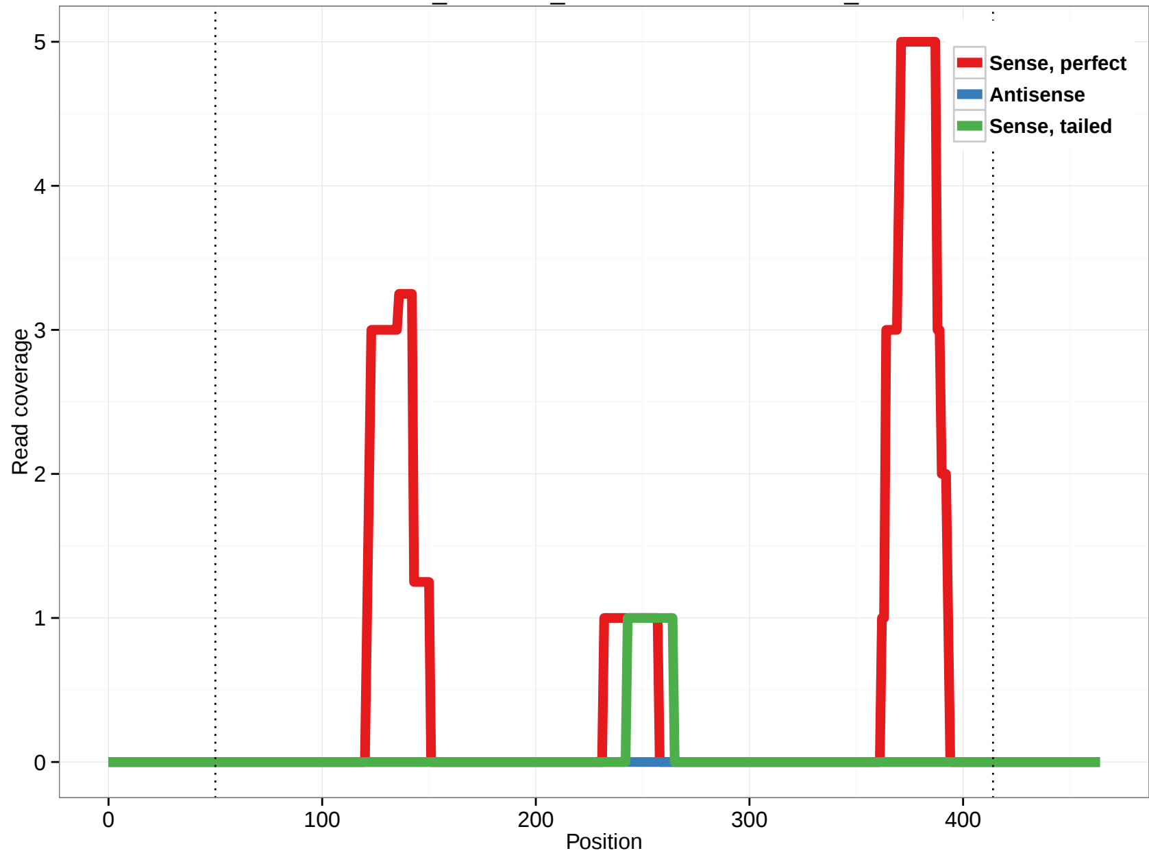
ornAna1_ensGene_ENSOANT00000006363_0
