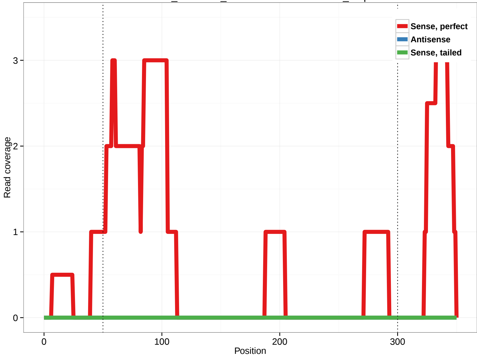
ornAna1_ensGene_ENSOANT00000006266_9.5p
