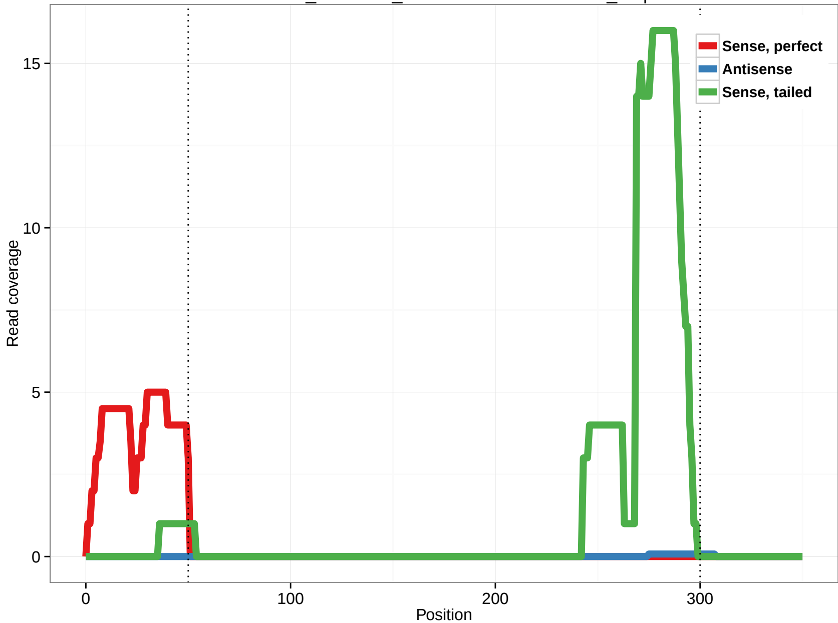
ornAna1_ensGene_ENSOANT00000006219_0.5p
