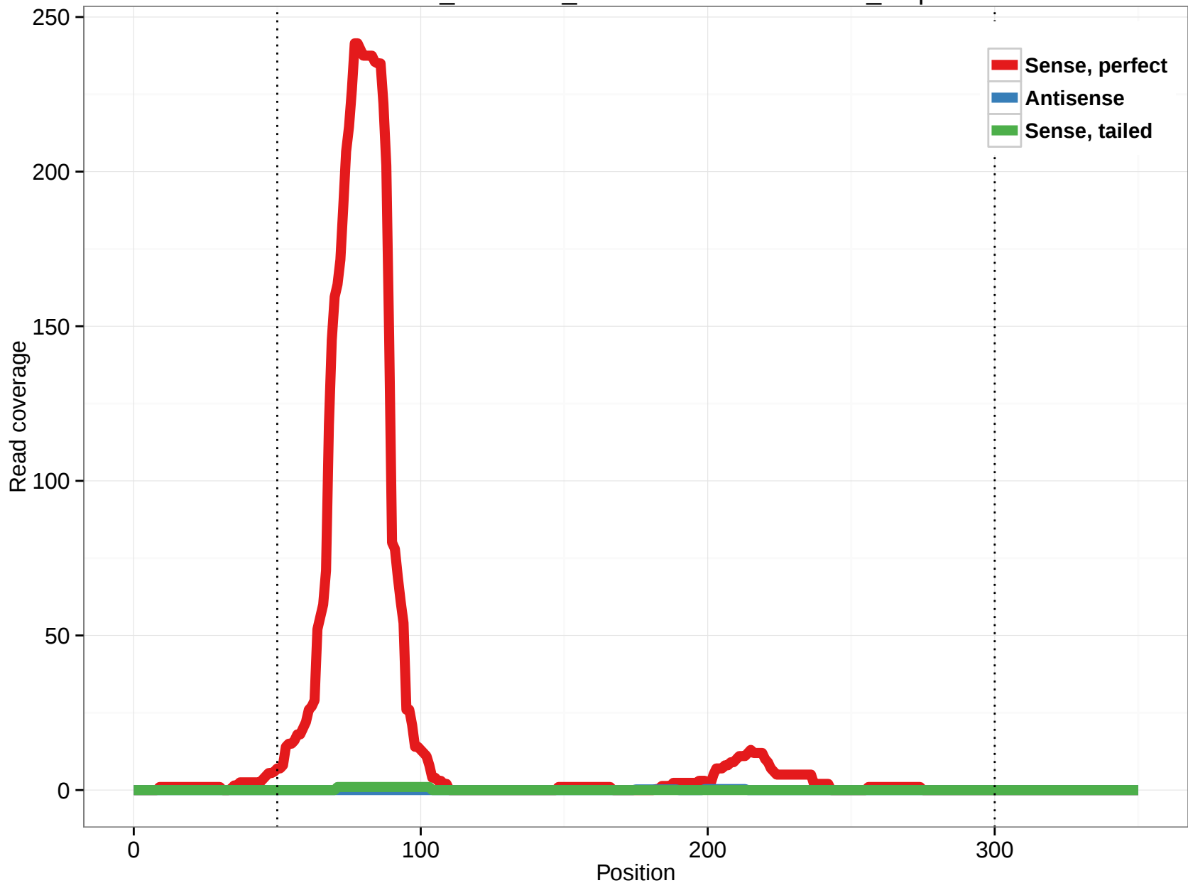
ornAna1_ensGene_ENSOANT00000006160_5.5p
