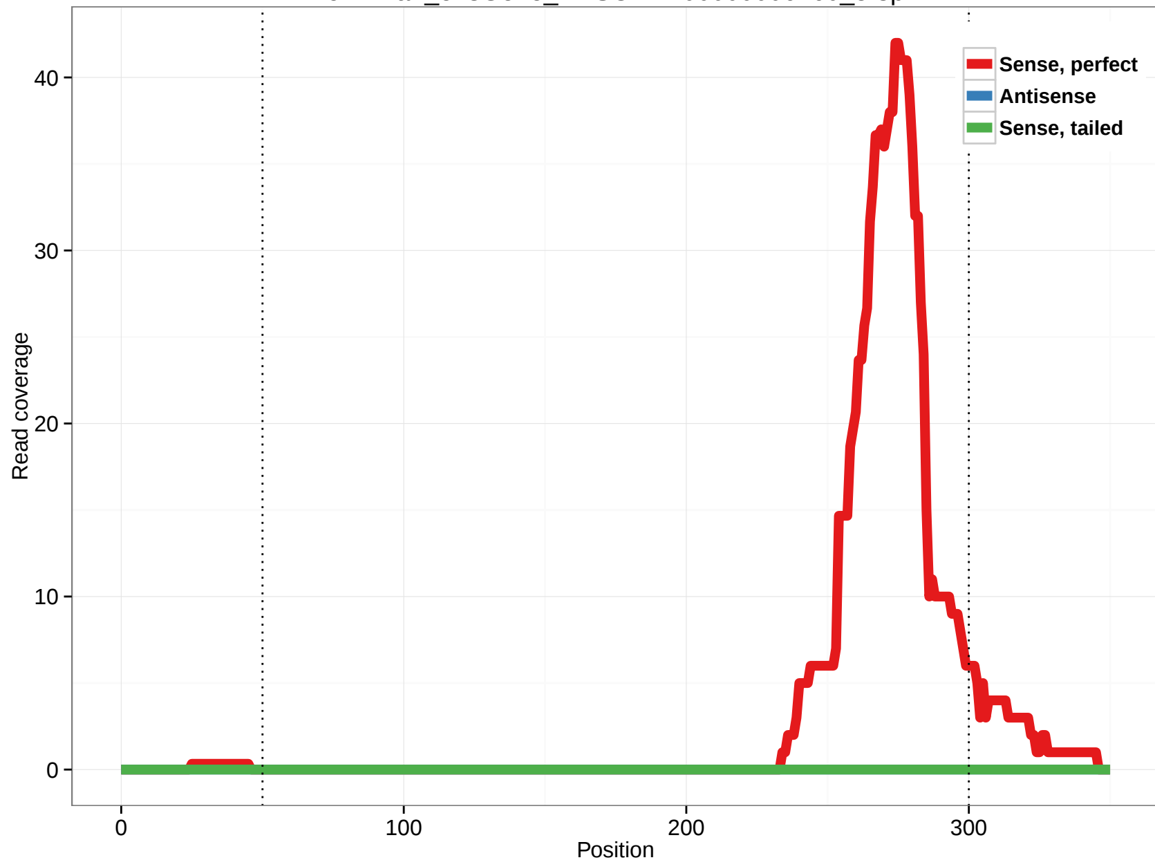
ornAna1_ensGene_ENSOANT00000006160_5.3p
