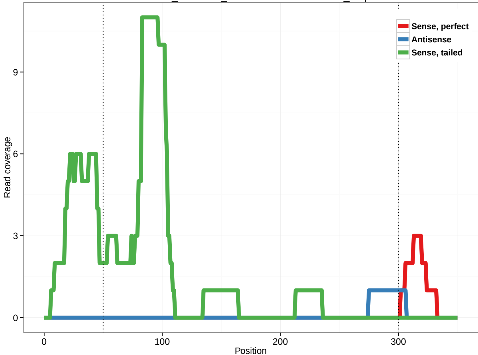
ornAna1_ensGene_ENSOANT00000006154_8.3p
