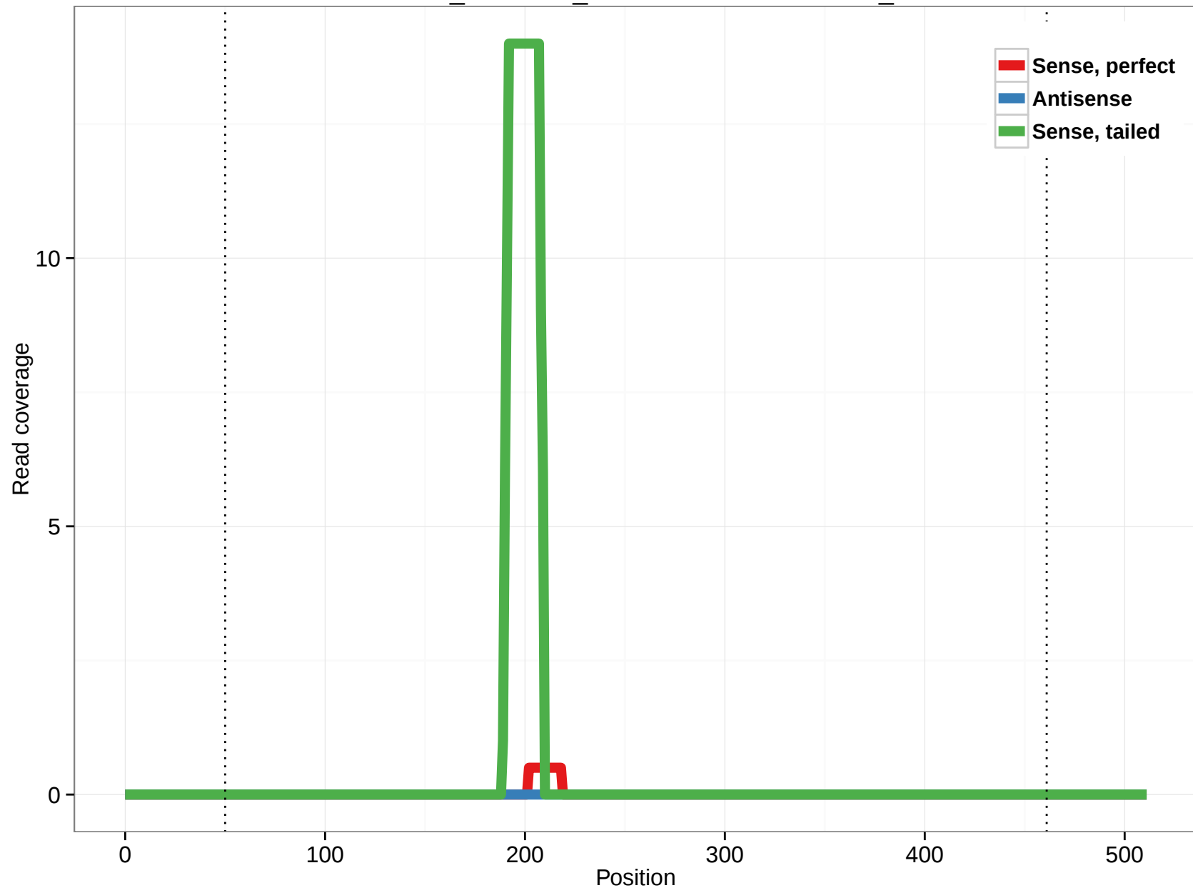
ornAna1_ensGene_ENSOANT00000006002_10
