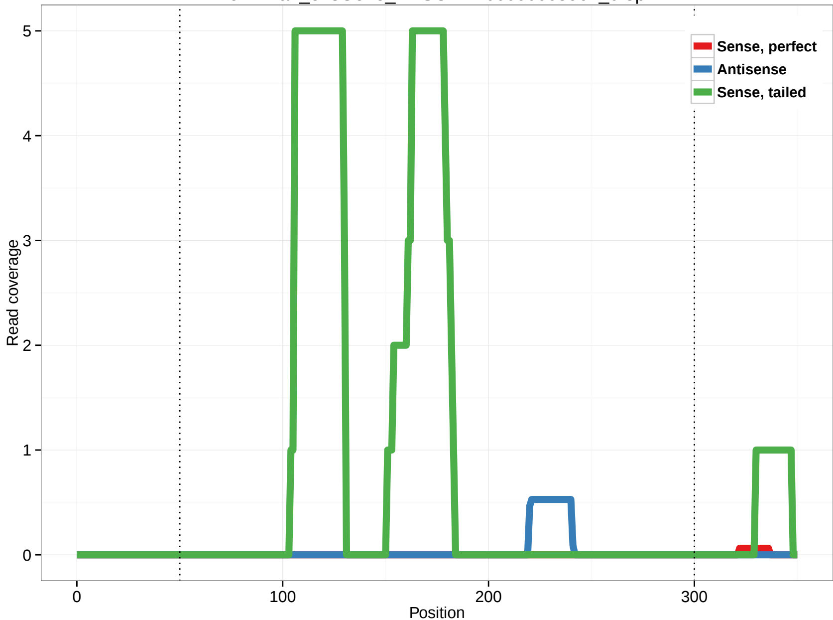
ornAna1_ensGene_ENSOANT00000005964_0.3p
