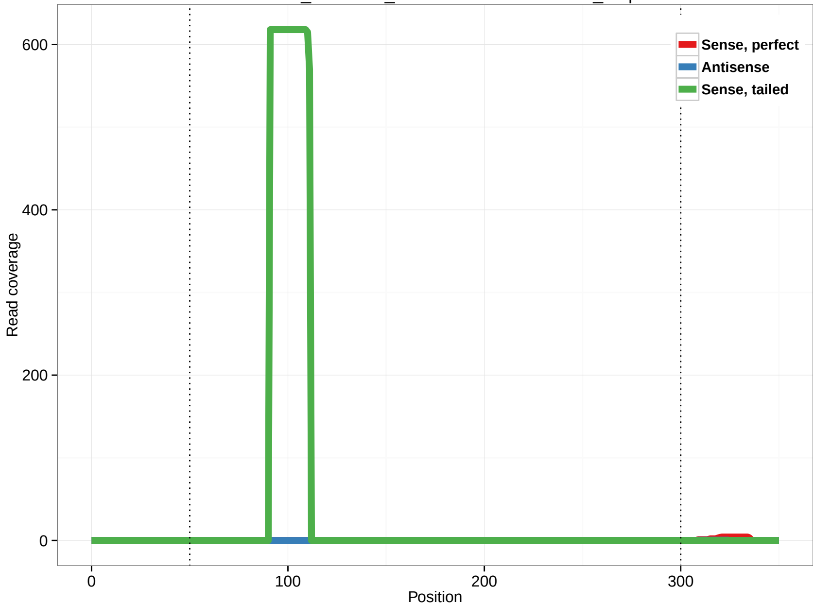
ornAna1_ensGene_ENSOANT00000005934_0.3p
