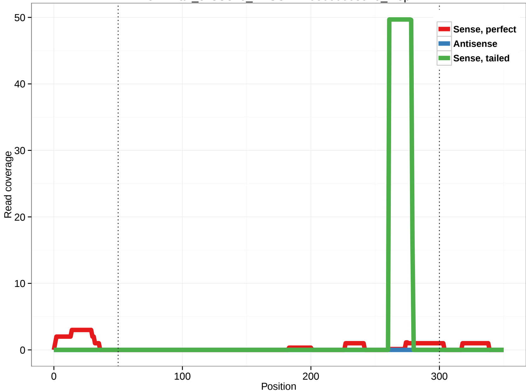
ornAna1_ensGene_ENSOANT00000005919_7.5p
