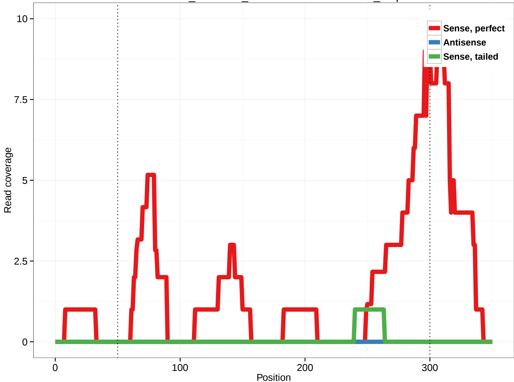
ornAna1_ensGene_ENSOANT00000005890_0.5p
