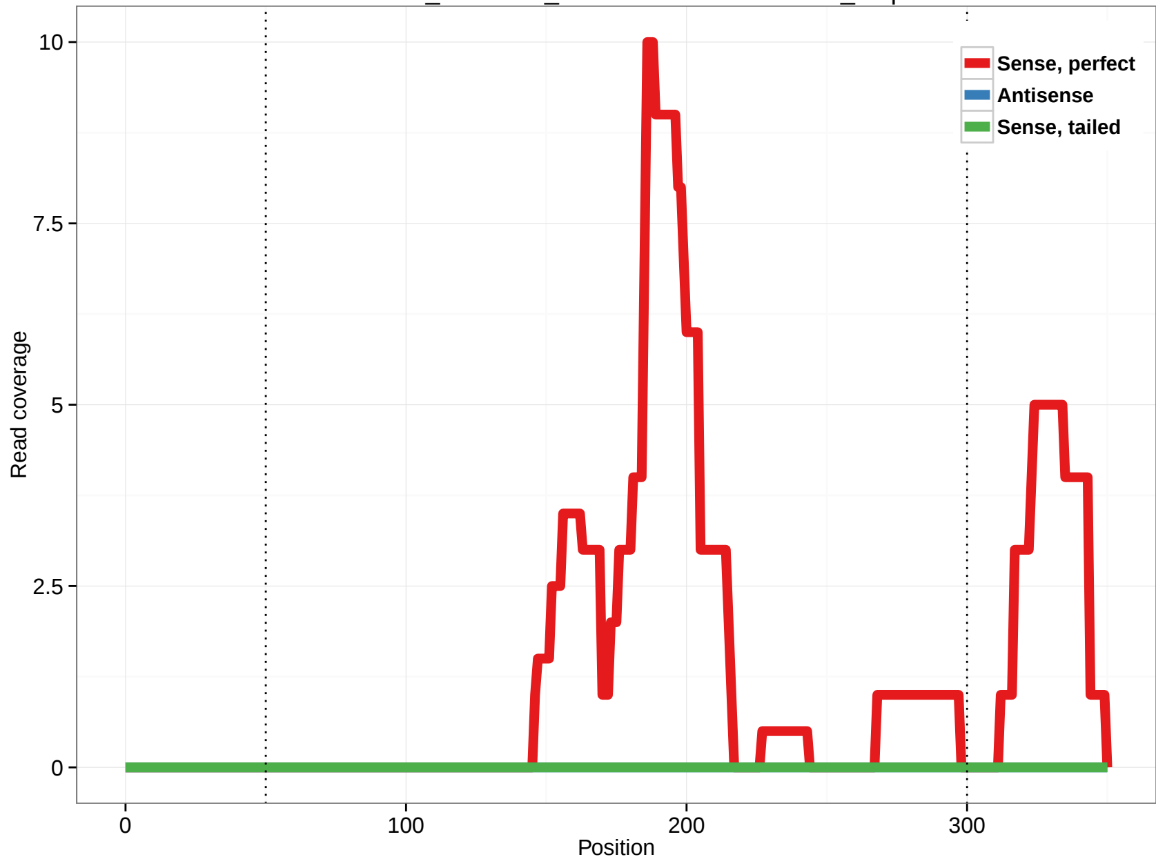
ornAna1_ensGene_ENSOANT00000005890_0.3p
