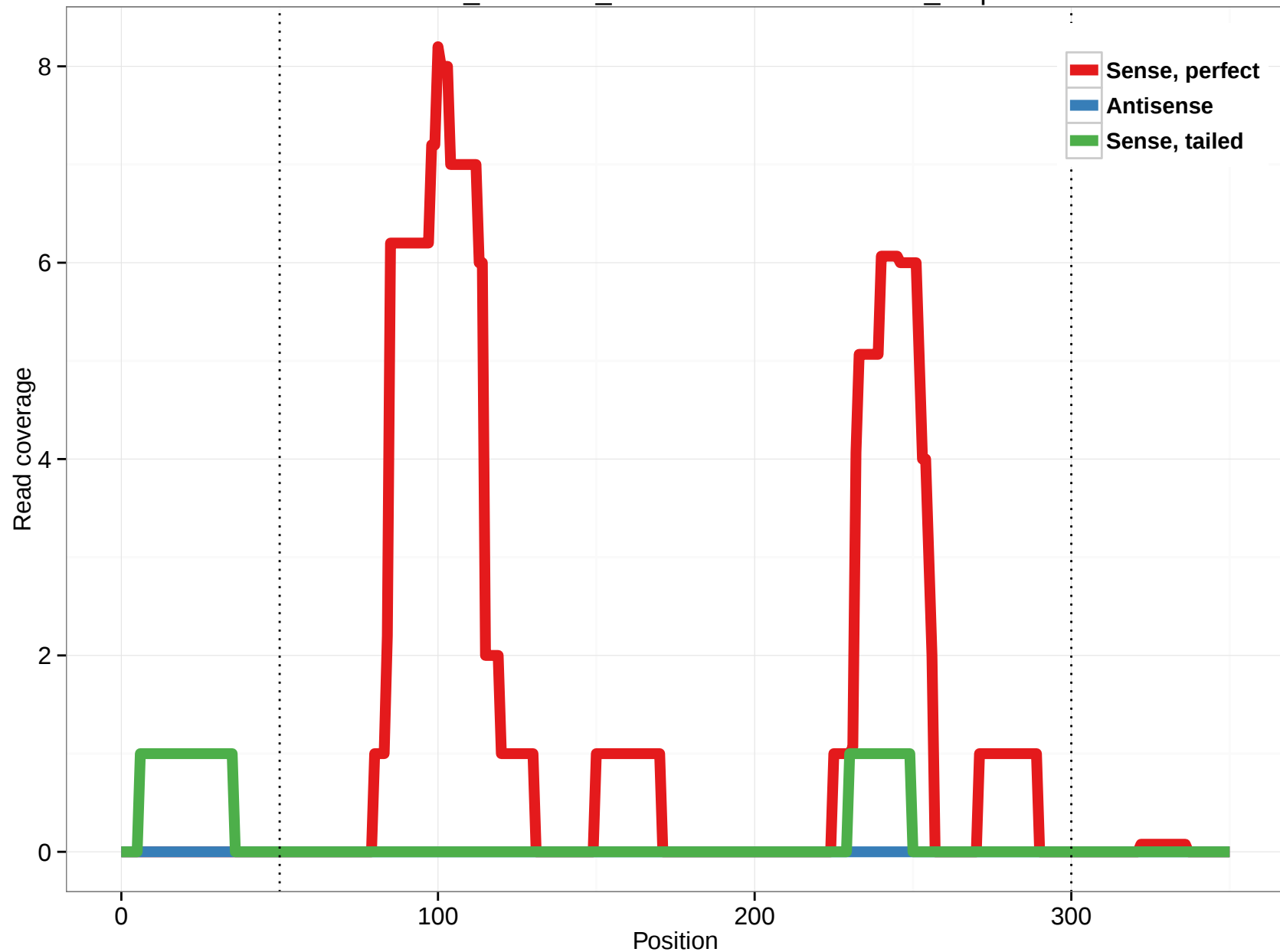
ornAna1_ensGene_ENSOANT00000005856_7.3p
