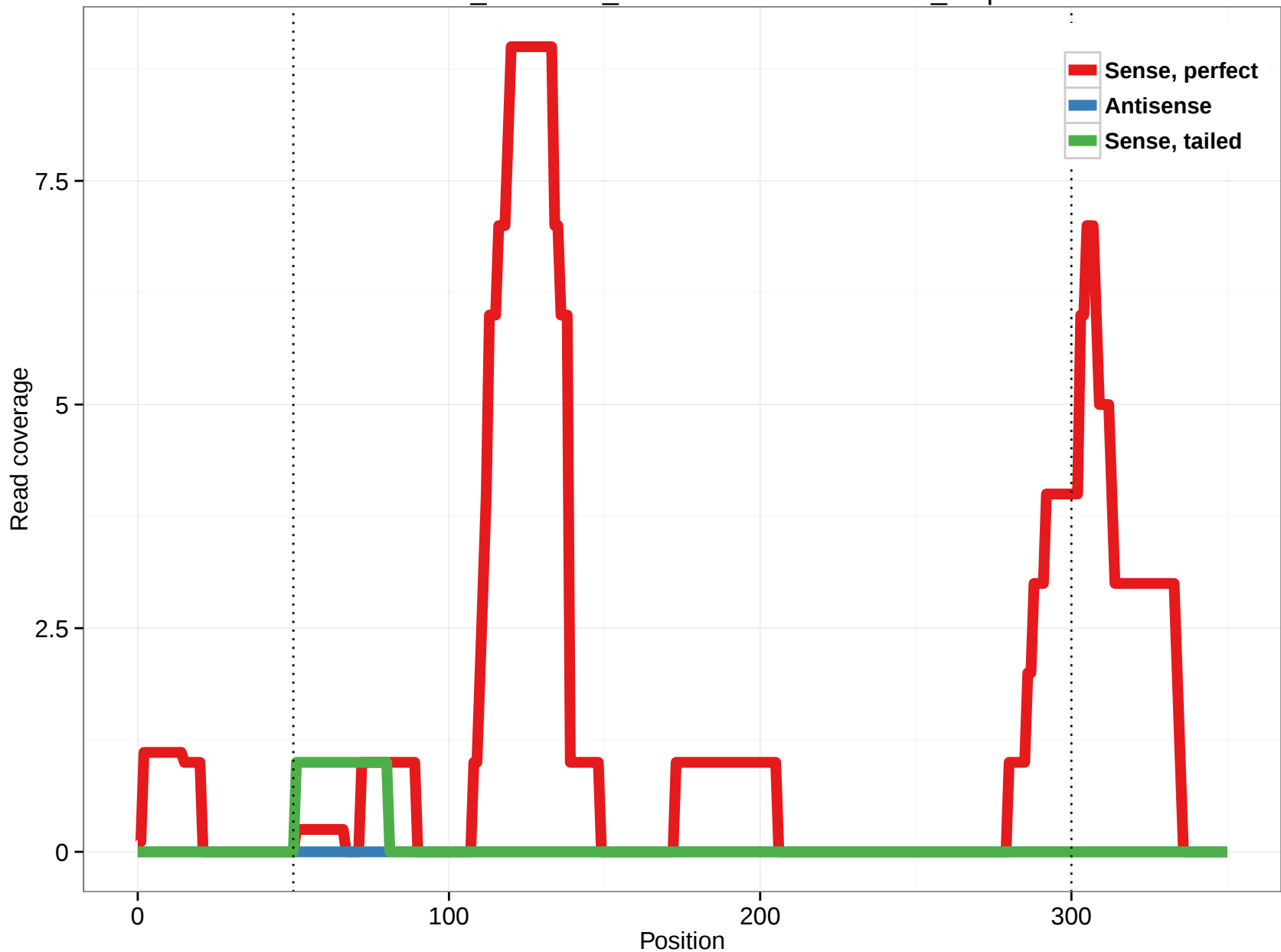
ornAna1_ensGene_ENSOANT00000005855_7.5p
