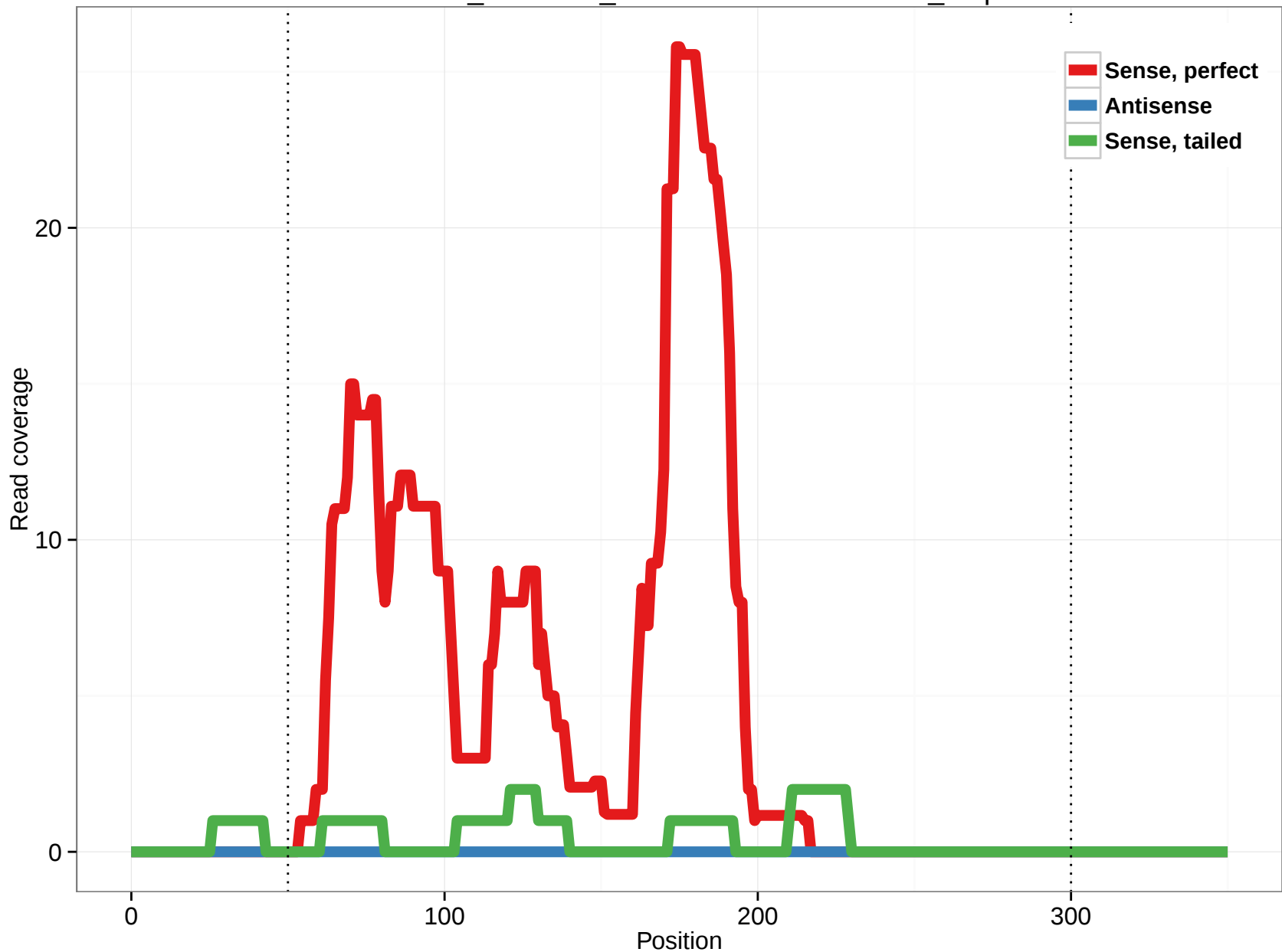
ornAna1_ensGene_ENSOANT00000005807_4.5p
