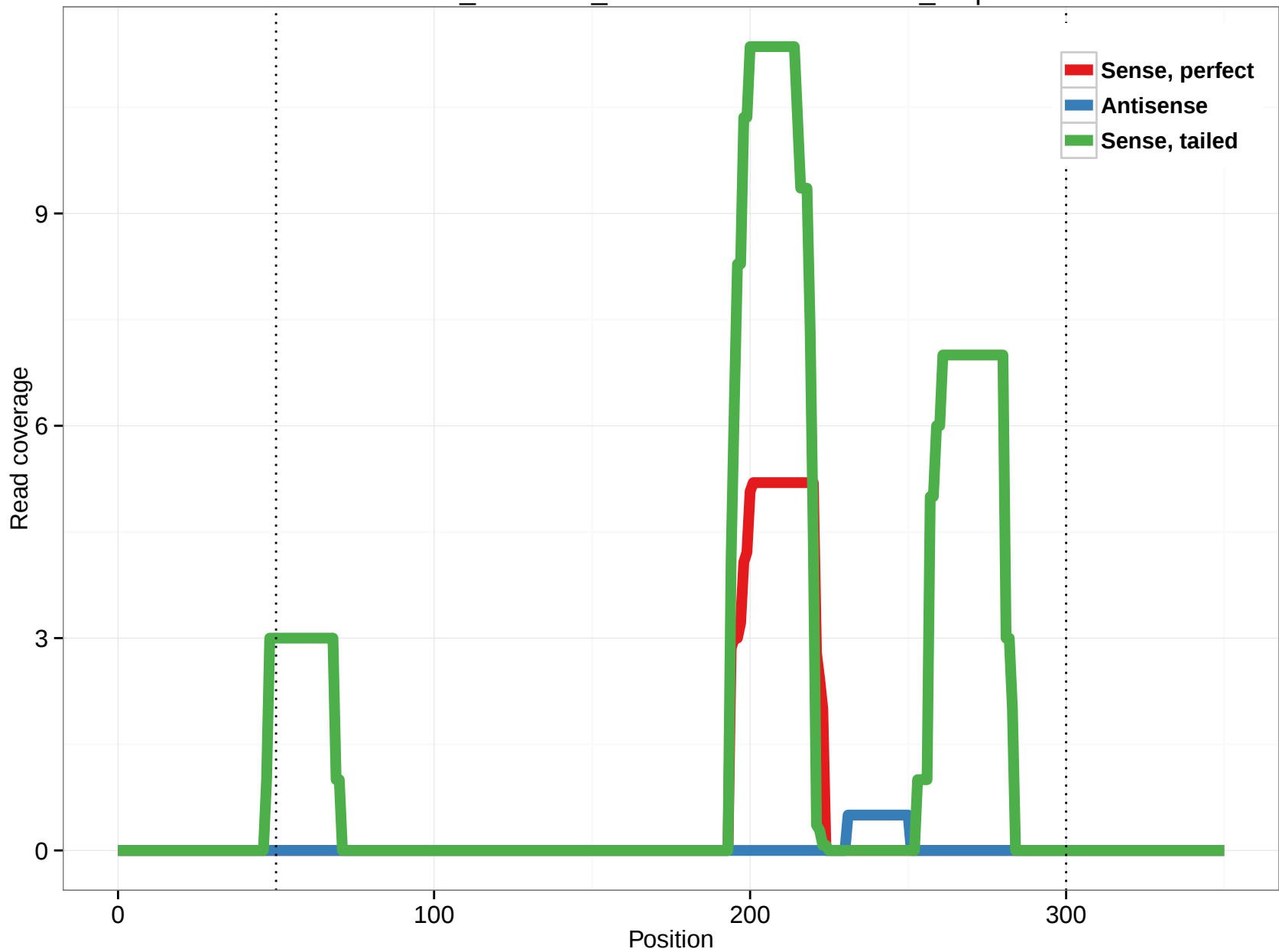
ornAna1_ensGene_ENSOANT00000005807_2.3p
