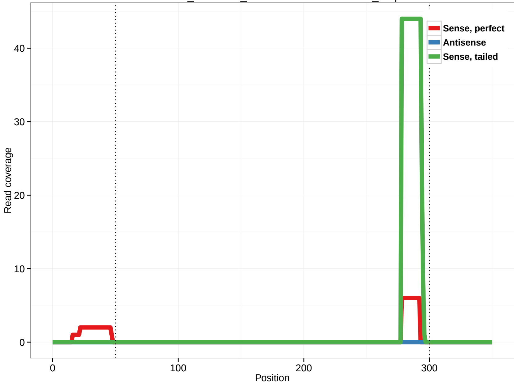
ornAna1_ensGene_ENSOANT00000005754_5.5p
