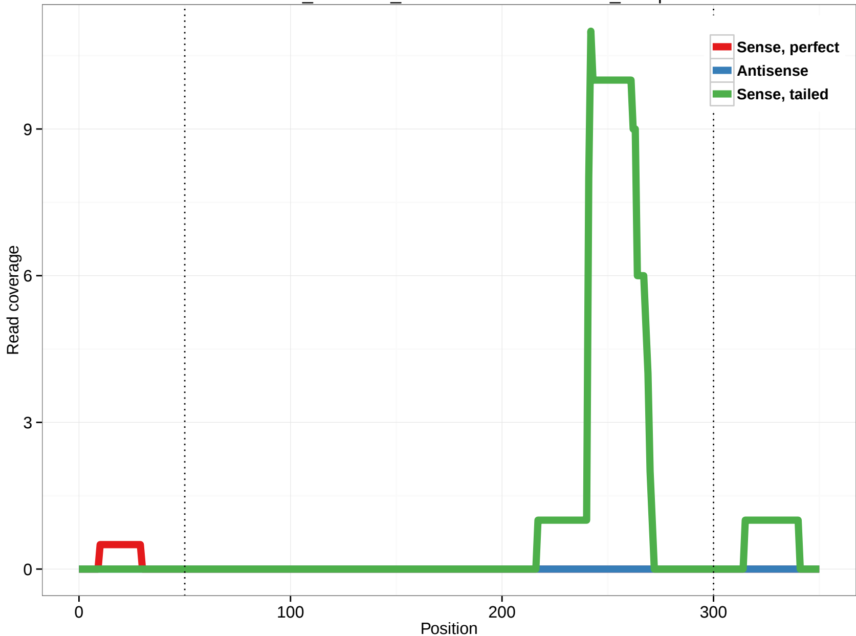
ornAna1_ensGene_ENSOANT00000005754_12.5p
