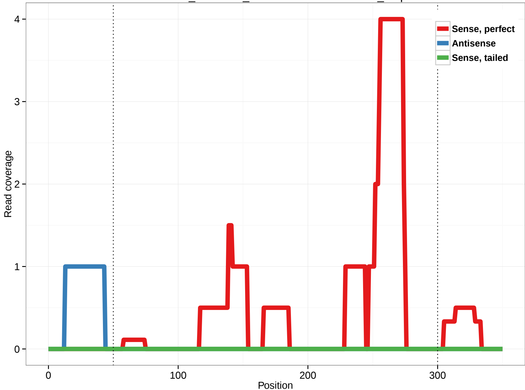
ornAna1_ensGene_ENSOANT00000005740_1.3p
