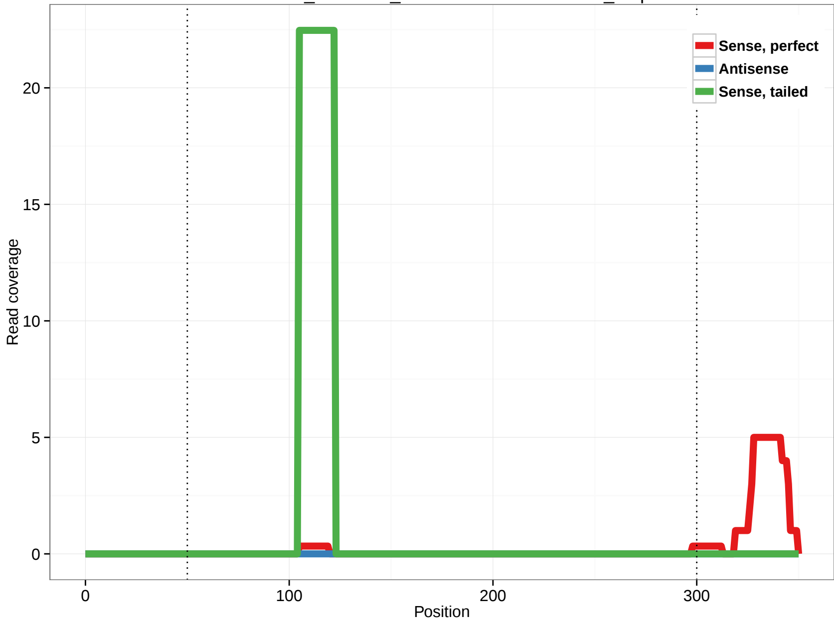
ornAna1_ensGene_ENSOANT00000005722_3.3p
