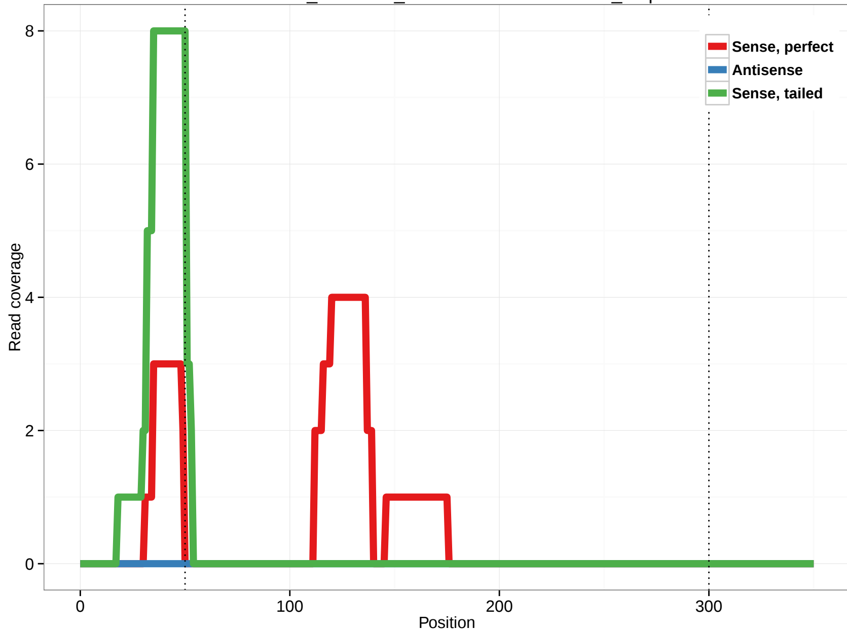
ornAna1_ensGene_ENSOANT00000005698_7.5p
