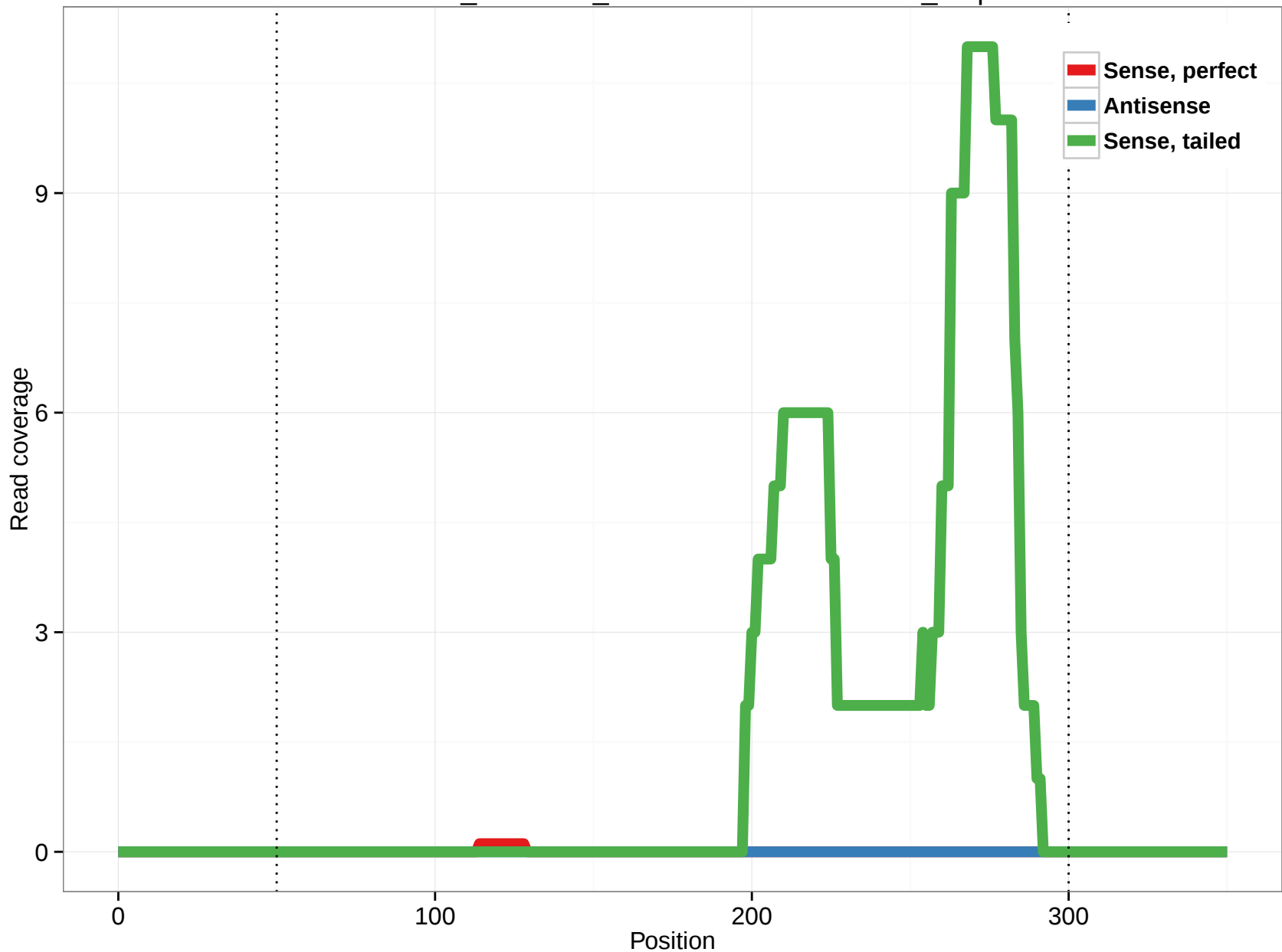
ornAna1_ensGene_ENSOANT00000005674_4.5p
