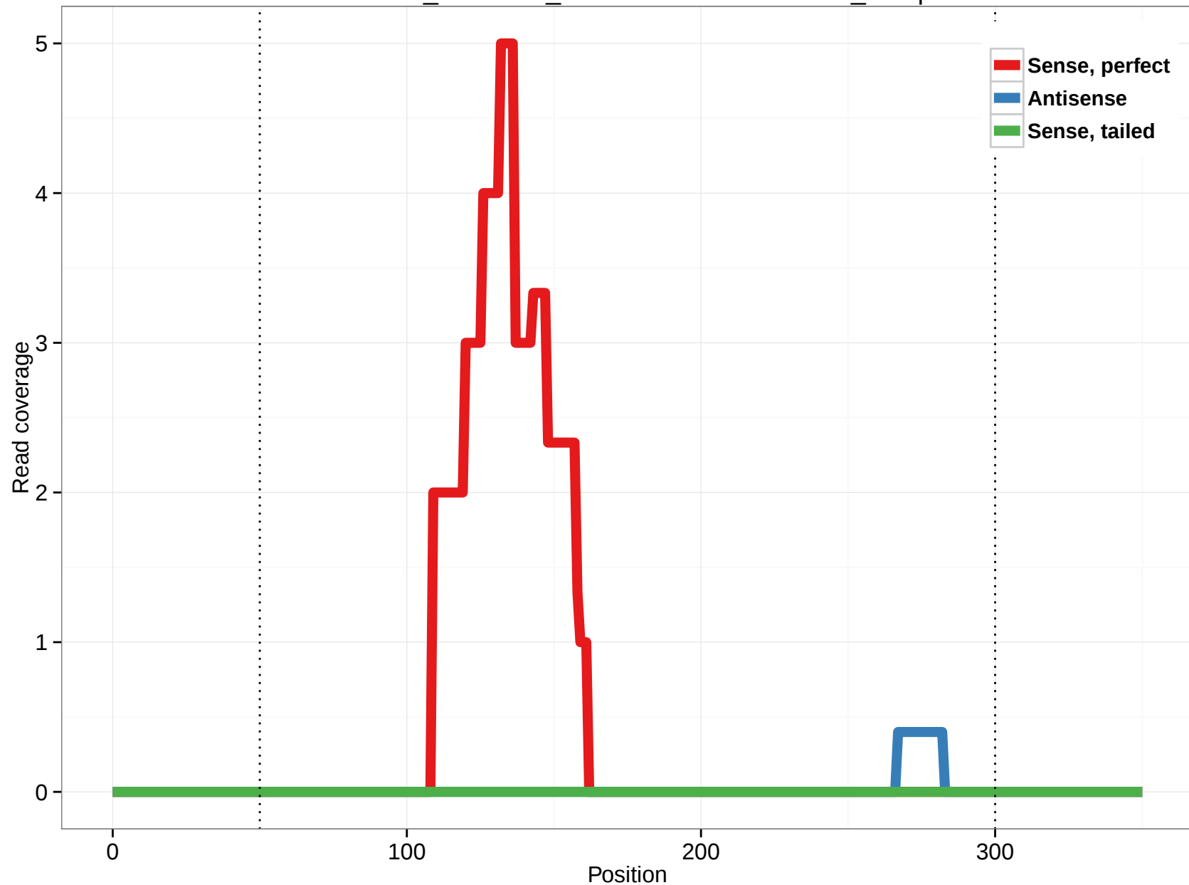
ornAna1_ensGene_ENSOANT00000005621_25.3p
