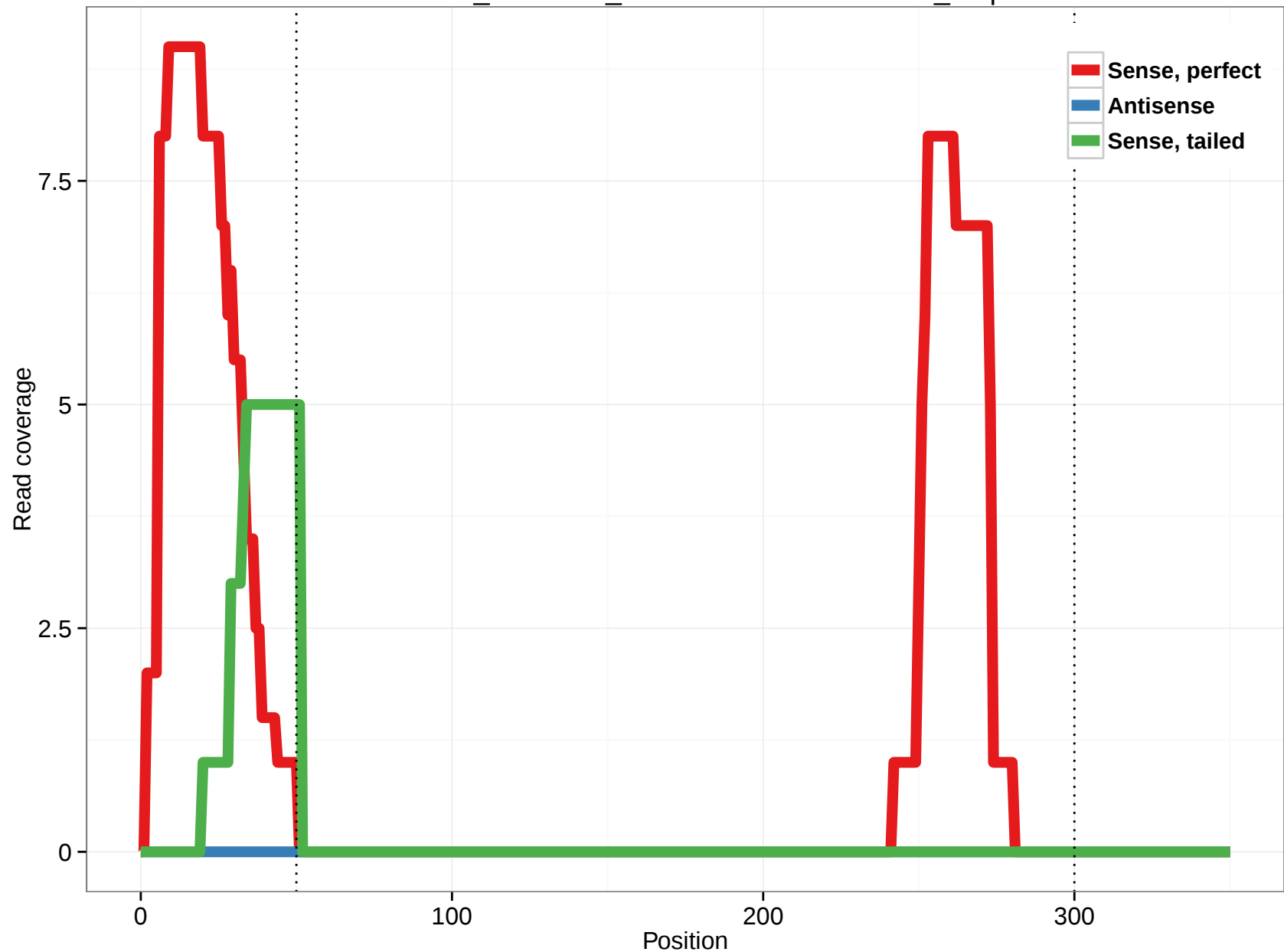
ornAna1_ensGene_ENSOANT00000005522_2.5p
