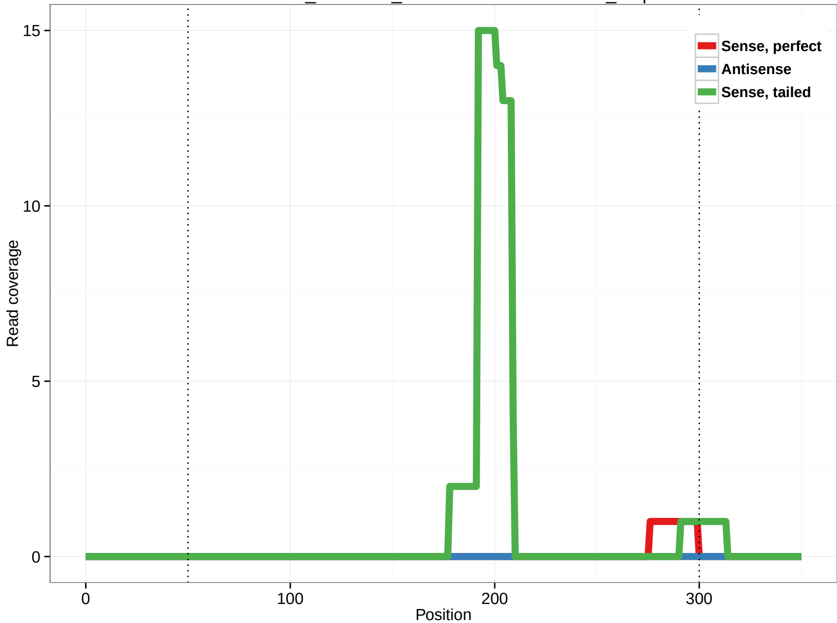
ornAna1_ensGene_ENSOANT00000005512_0.5p
