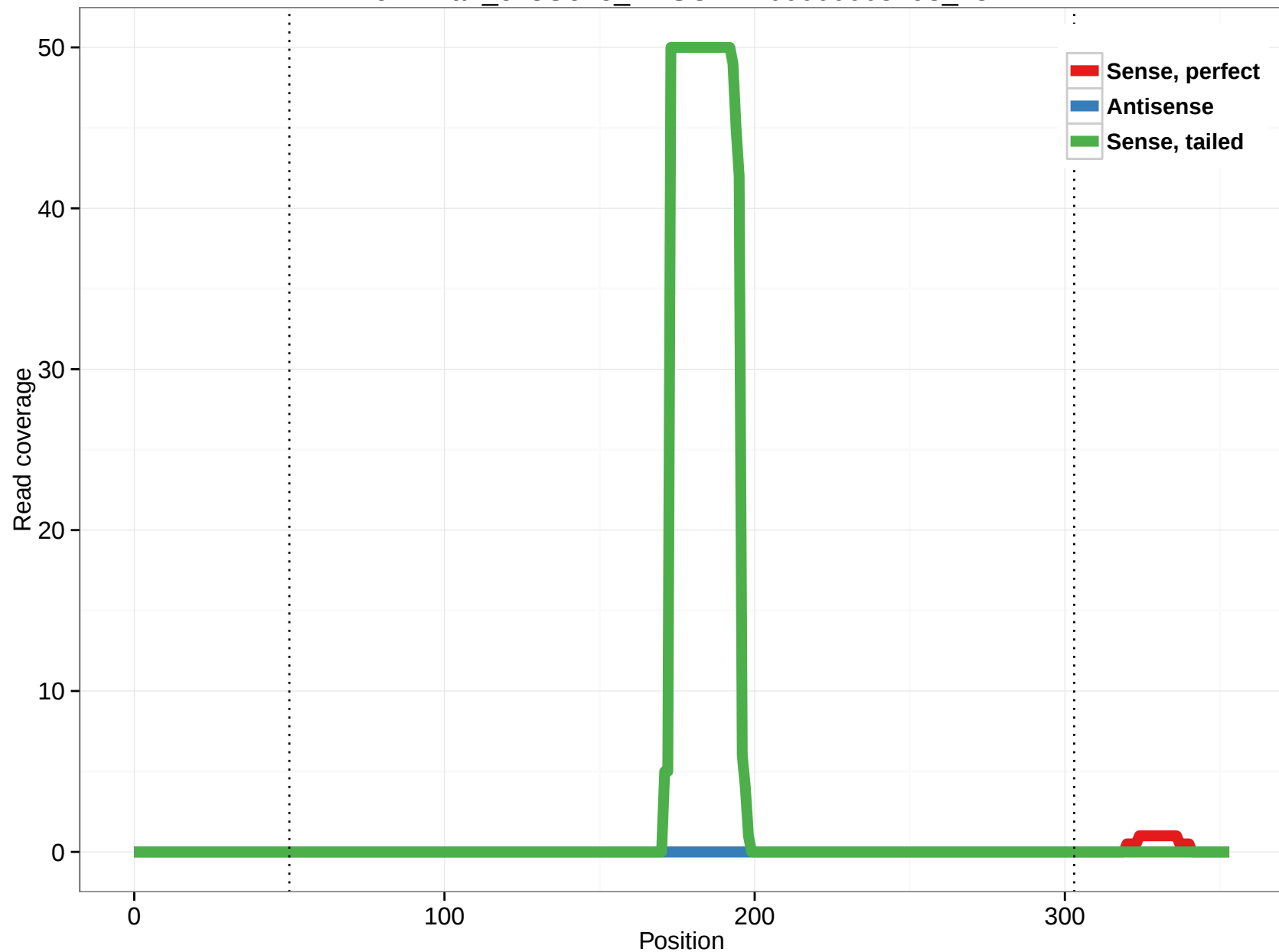
ornAna1_ensGene_ENSOANT00000005493_13
