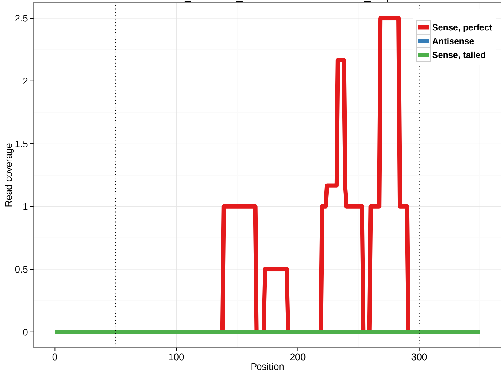
ornAna1_ensGene_ENSOANT00000005384_3.5p
