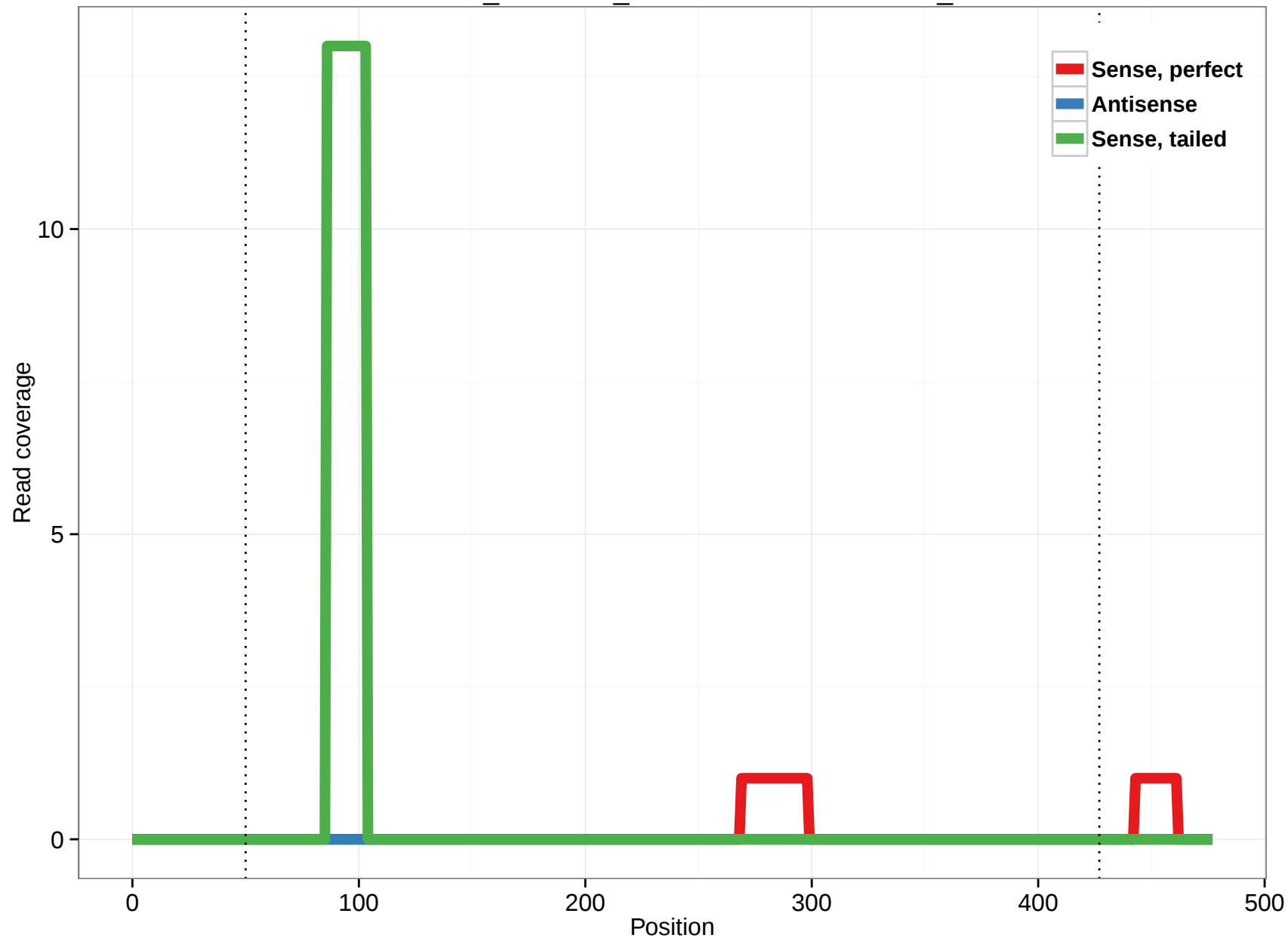
ornAna1_ensGene_ENSOANT00000005367_4
