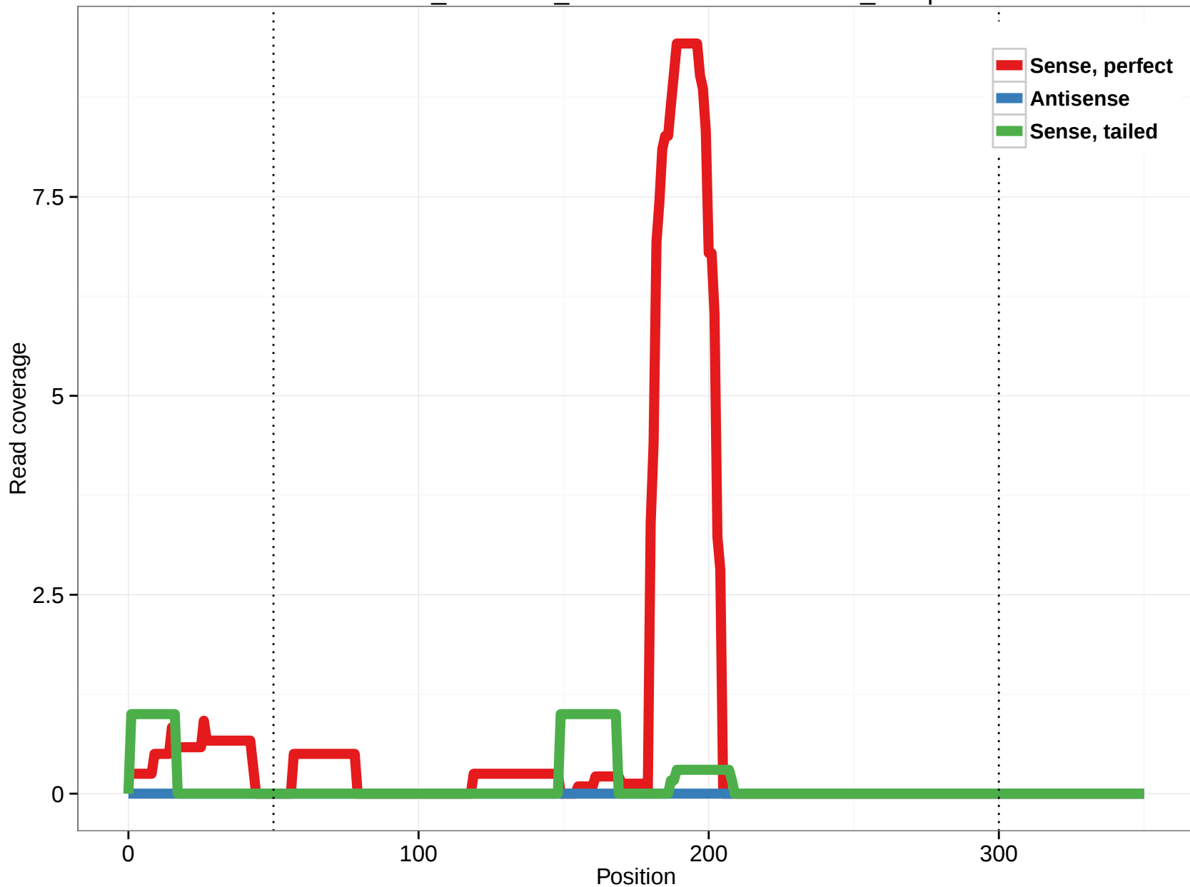
ornAna1_ensGene_ENSOANT00000005360_34.5p
