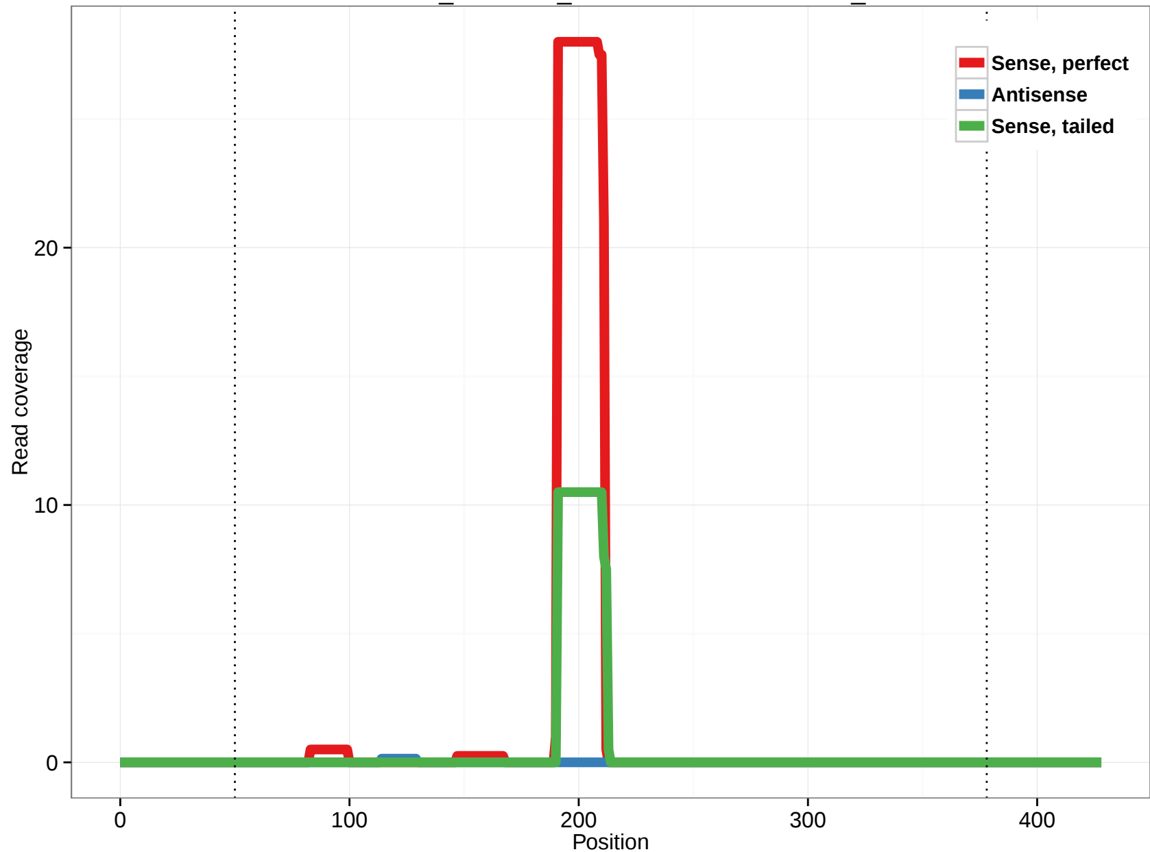
ornAna1_ensGene_ENSOANT00000005357_9
