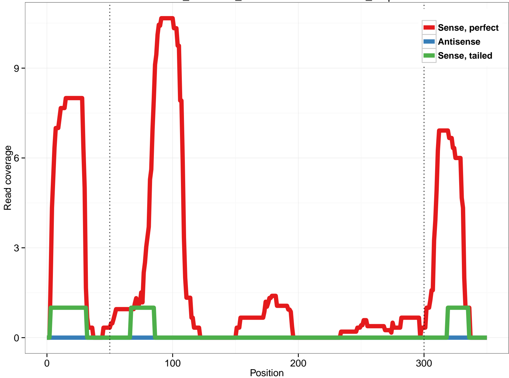
ornAna1_ensGene_ENSOANT00000005310_0.3p
