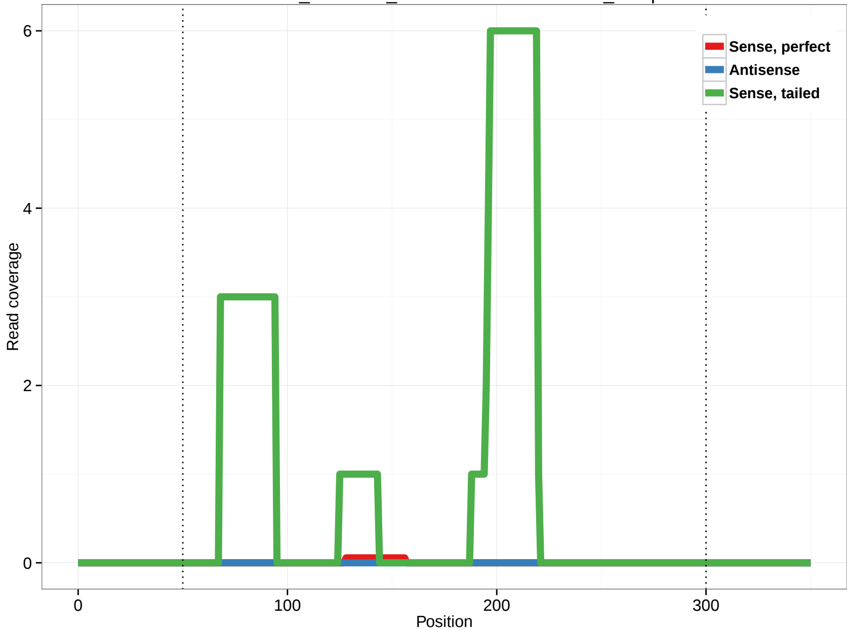
ornAna1_ensGene_ENSOANT00000005309_17.5p
