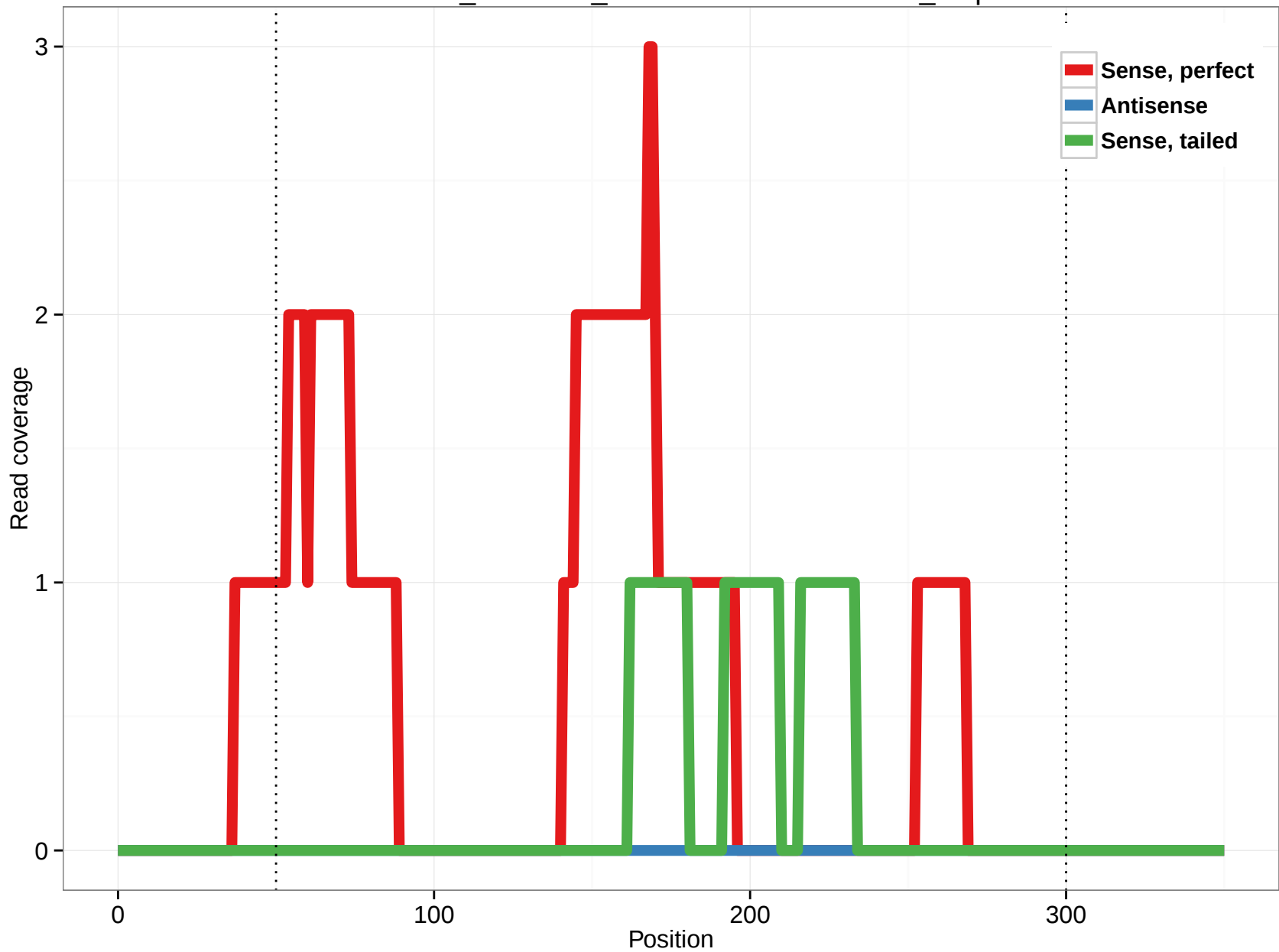
ornAna1_ensGene_ENSOANT00000005294_2.3p
