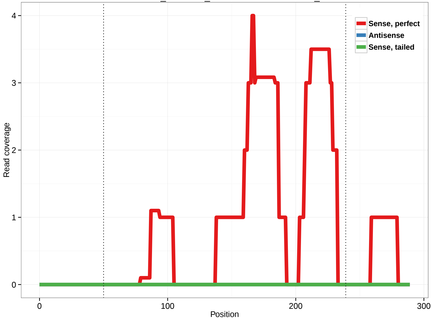
ornAna1_ensGene_ENSOANT00000005293_5
