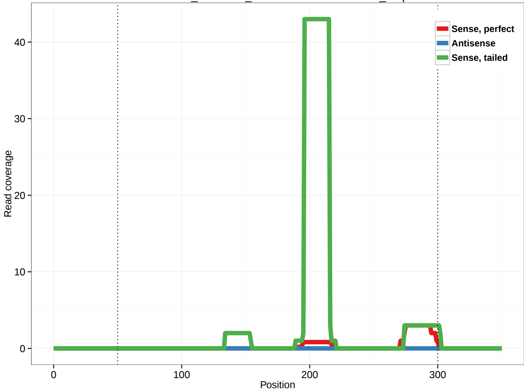
ornAna1_ensGene_ENSOANT00000005275_9.5p
