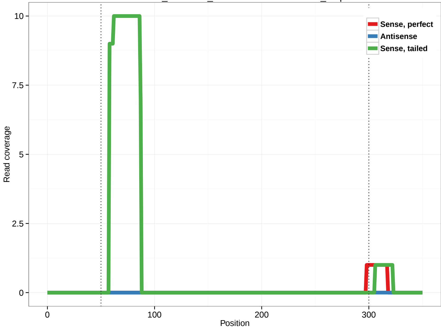
ornAna1_ensGene_ENSOANT00000005224_1.3p
