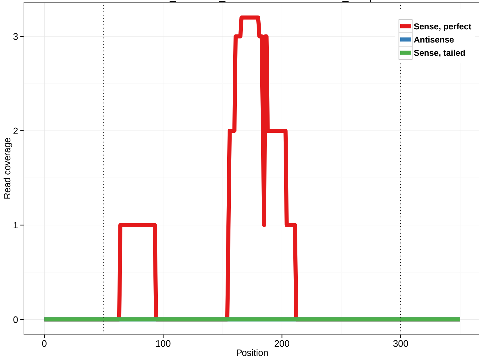
ornAna1_ensGene_ENSOANT00000005201_16.3p
