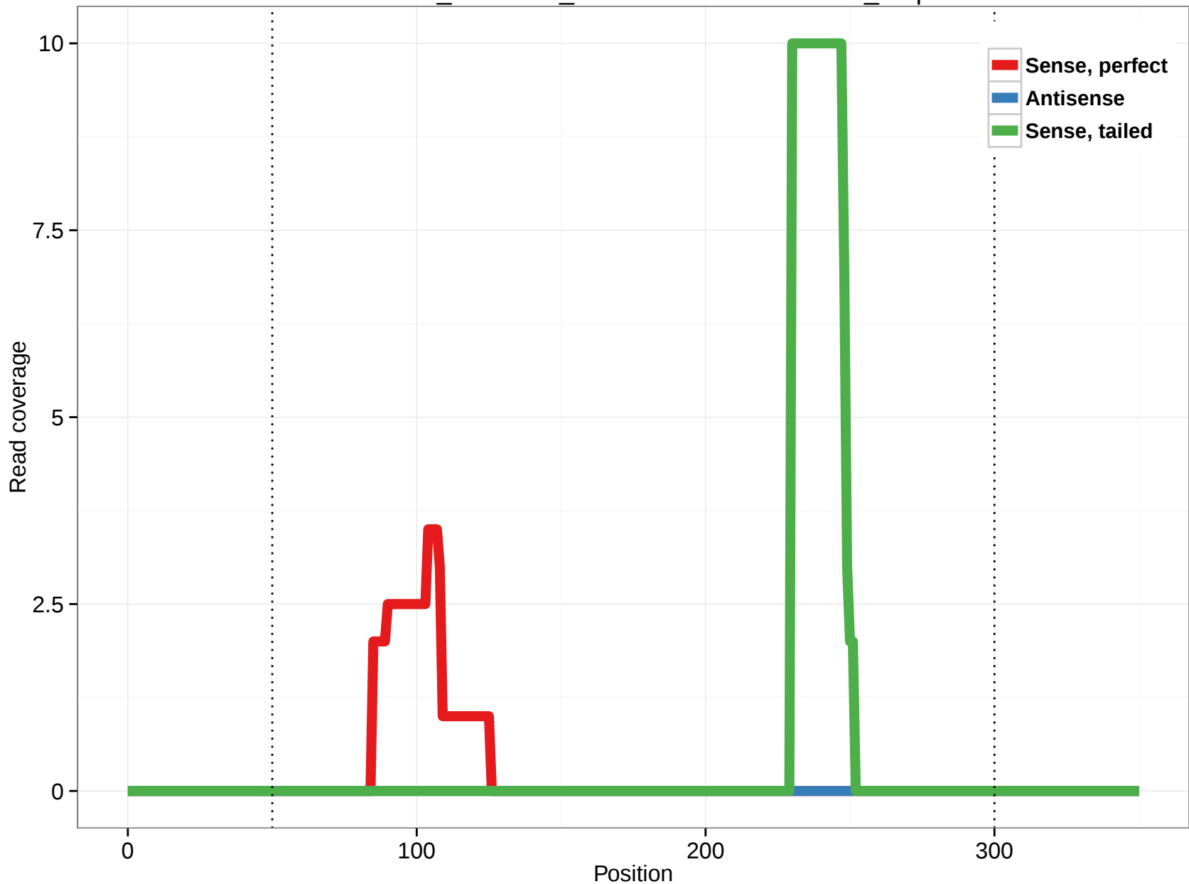
ornAna1_ensGene_ENSOANT00000005175_3.5p
