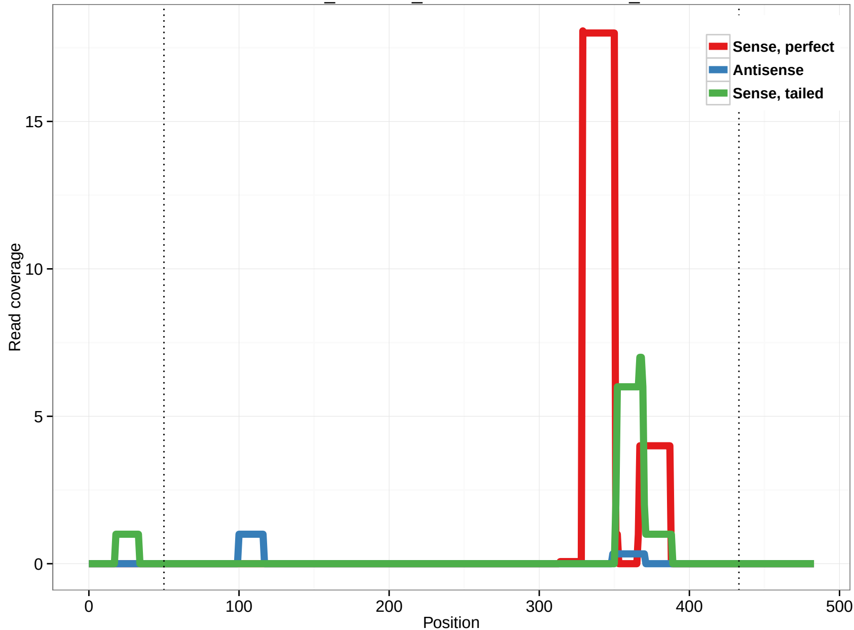
ornAna1_ensGene_ENSOANT00000005151_4
