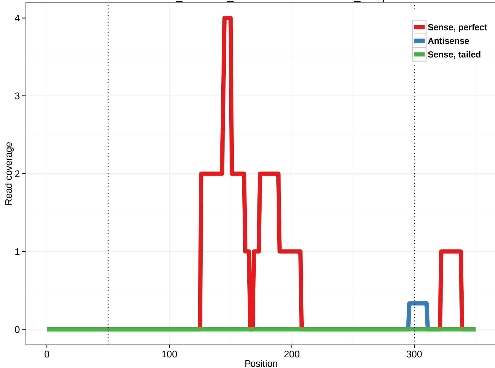
ornAna1_ensGene_ENSOANT00000005127_21.3p
