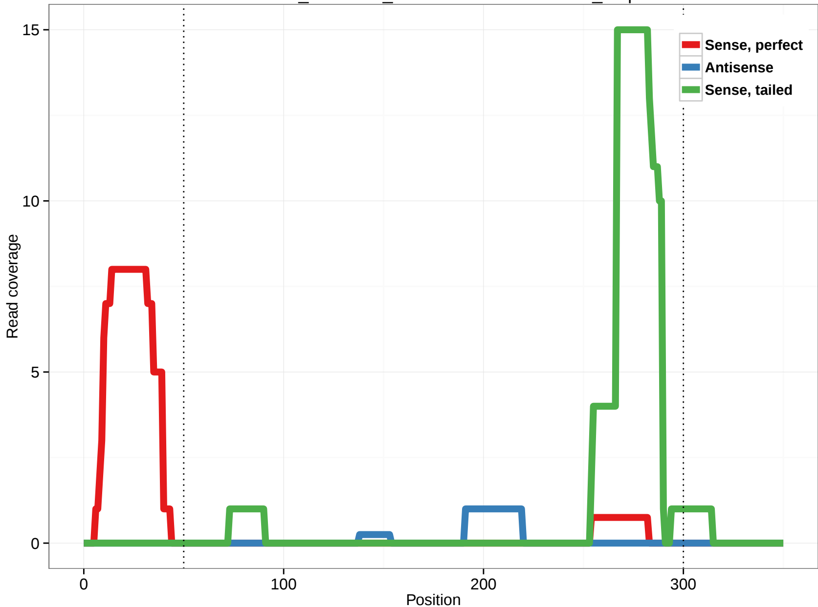
ornAna1_ensGene_ENSOANT00000005126_0.5p
