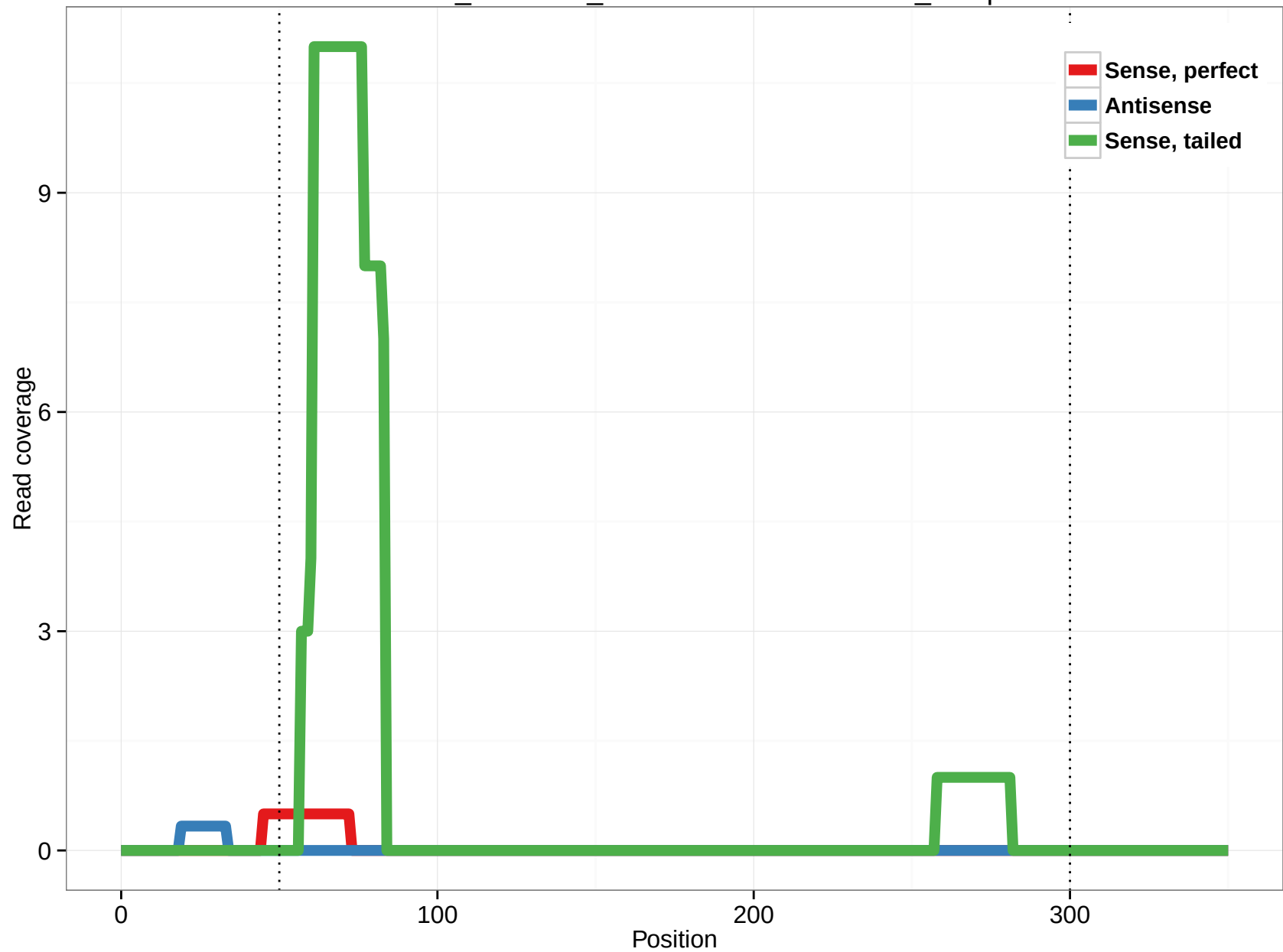
ornAna1_ensGene_ENSOANT00000005086_17.3p
